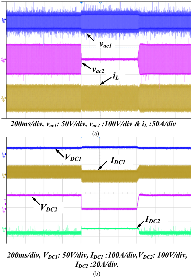
Fig. 8. Experimental waveforms showing short circuit DC fault on HV (100V) terminal (a) AC voltages and currents (b) DC voltages and currents
