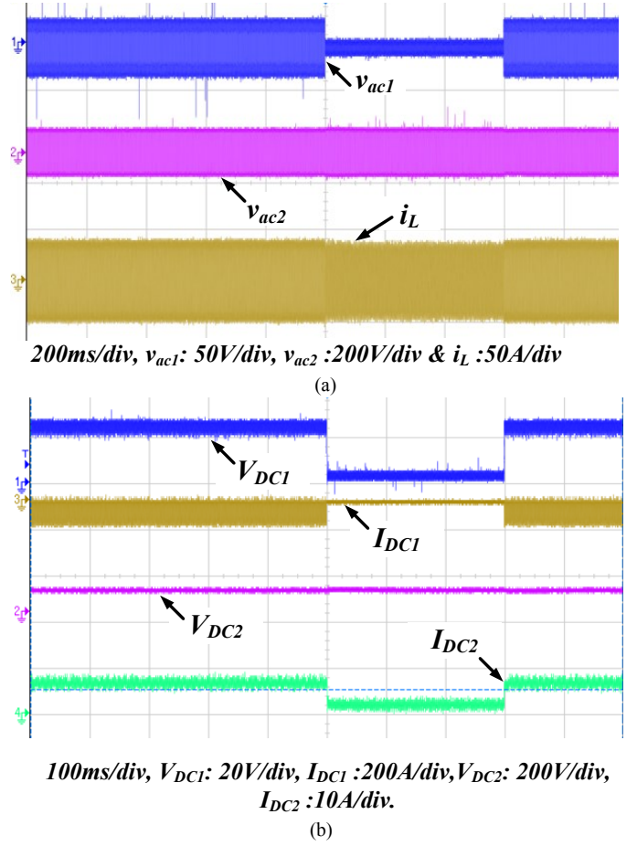
Fig. 7. Experimental waveforms showing short circuit DC fault on LV (24V) terminal (a) AC voltages and currents (b) DC voltages and currents
