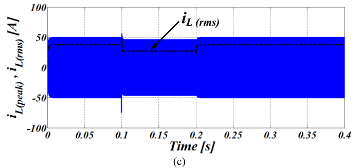
Fig. 3. Simulation results showing DC fault on LV side (a) Bridge 1 AC voltage v_{ac1} , (b) Bridge 2 AC voltage v_{ac2} , (c) Inductor current i_L .
