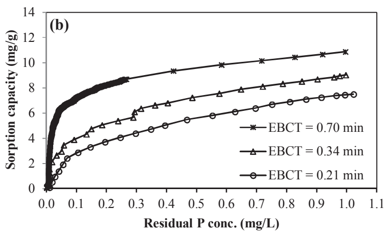
Fig. 2 – Effect of EBCT on phosphate sorption by Mg-Fe-Cl LDH in fixed bed column test: (a) breakthrough curves; (b) sorption capacity.
