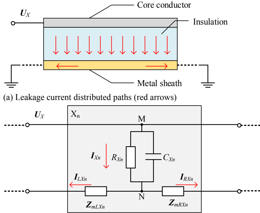
Fig. 4. Leakage current paths and model for an XLPE insulated minor section
