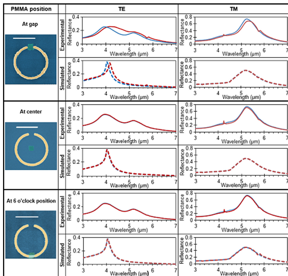
FIG. 3. Experimental and simulated spectra of the SRR array with a 150 nm by 150 nm block of PMMA (110 nm thick) localized in three different positions—at the gap of the SRR, in the center of the SRR, and at the “6 o’clock” position on the arm of the SRR. The blue plots show the spectra of the SRRs alone and red plots with localized PMMA. SEM micrographs with false color show the position of the PMMA (green) with respect to the SRR (gold) on the silica substrate (blue). The white scale bar represents a length of 1 \mu m.
