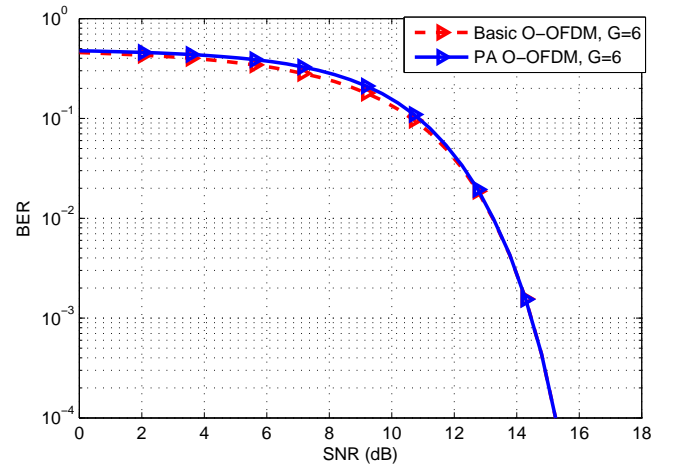
Fig. 4: BER plot of basic and PA O-OFDM with multiple LEDs using G = 6 , U = 5 , P = 5
