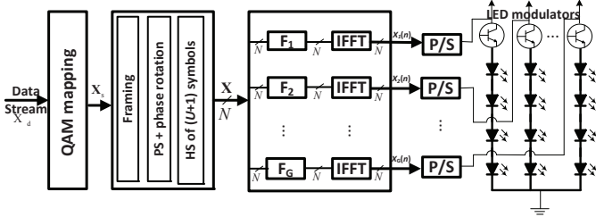
Fig. 2: Block diagram illustrating the transmitter architecture of pilot-assisted O-OFDM system with multiple LED groups.
