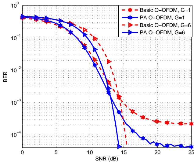
Fig. 5: BER performance of basic and PA O-OFDM system with and without grouped LEDs using U = 5 , P = 5 , G = 1, 6 , \mathcal{D} = 96 and N = 194 . The levels are set to \sigma_x = 250 mA, c_u = c_l = 1 , \mathcal{B}_g = 250 mA and 220 mA for basic and PA system with G = 1 respectively; while \mathcal{B}_g = 40 mA and 30 mA for basic and PA system with G = 6 respectively.
