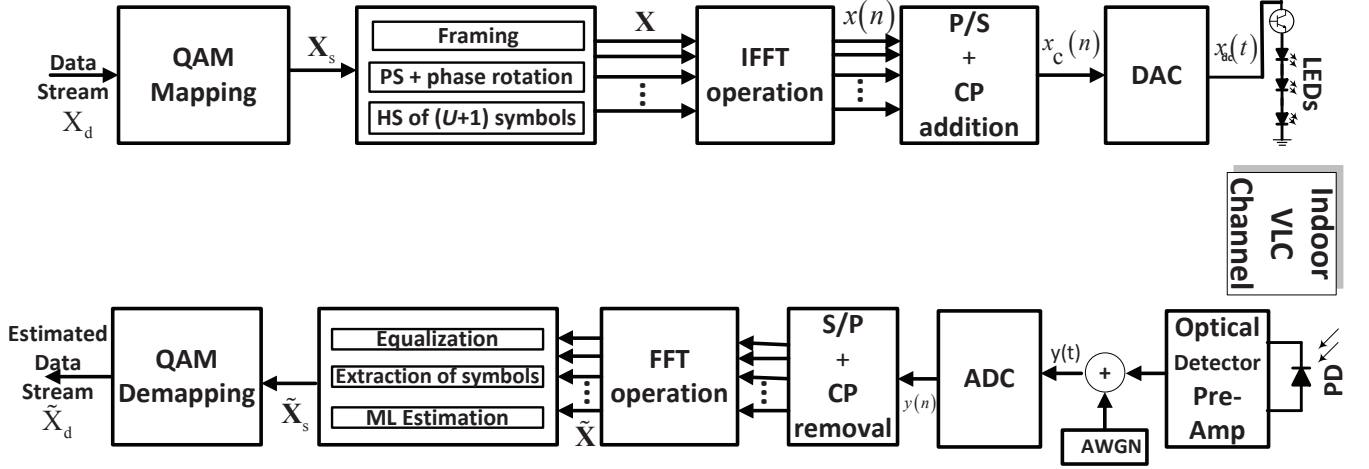
Fig. 1: Block diagram illustrating the pilot-assisted O-OFDM system. PS: pilot symbol; HS: Hermitian symmetry; P/S: Parallel-to-serial; S/P: serial-to-parallel; DAC: digital-to-analog converter; ADC: analog-to-digital converter
