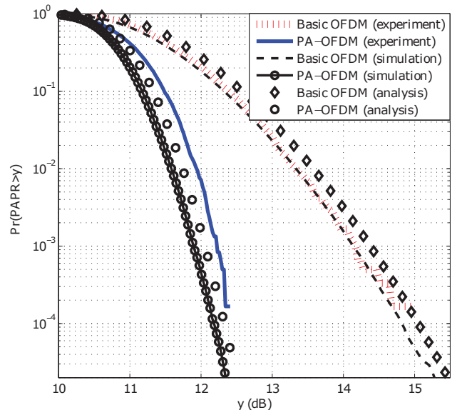
Fig. 4: CCDF plot for basic and PA-OFDM signal using 16-QAM, L = 4 , U = 5 , P = 5 , N = 256 , and equation (3).
