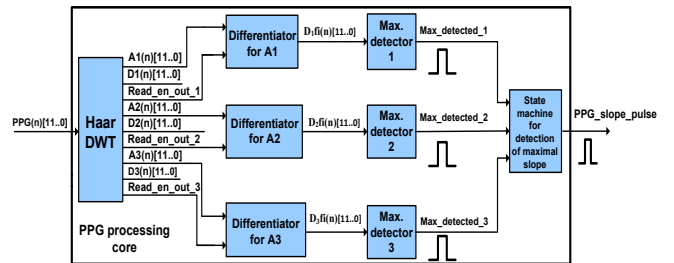
Fig. 9. Internal structure of PPG slope detection core.
