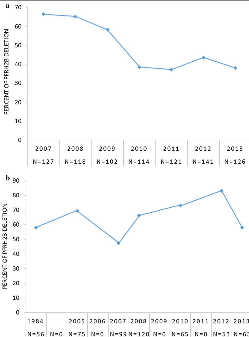
Fig. 1 Evolution of PFRh2b deletion in Thiès (a) and Western Gambia (b). Scheme showing the variation in the prevalence of PFRh2b deletion over the time, including mixed infections ( PFRh2 full-length and PFRh2b deletion) in both areas using formula described previously by Ahouidi et al. [10]. Alleles frequencies of the dimorphic PFRh2b gene were determined using semi-nested Polymerase Chain Reaction (PCR). a A decrease of PFRh2b deletion from 2007 to 2013 in Thiès was noted. b A fluctuation of this deletion from 1984 to 2013 in The Gambia was observed. N, number of isolates; Del, deletion
