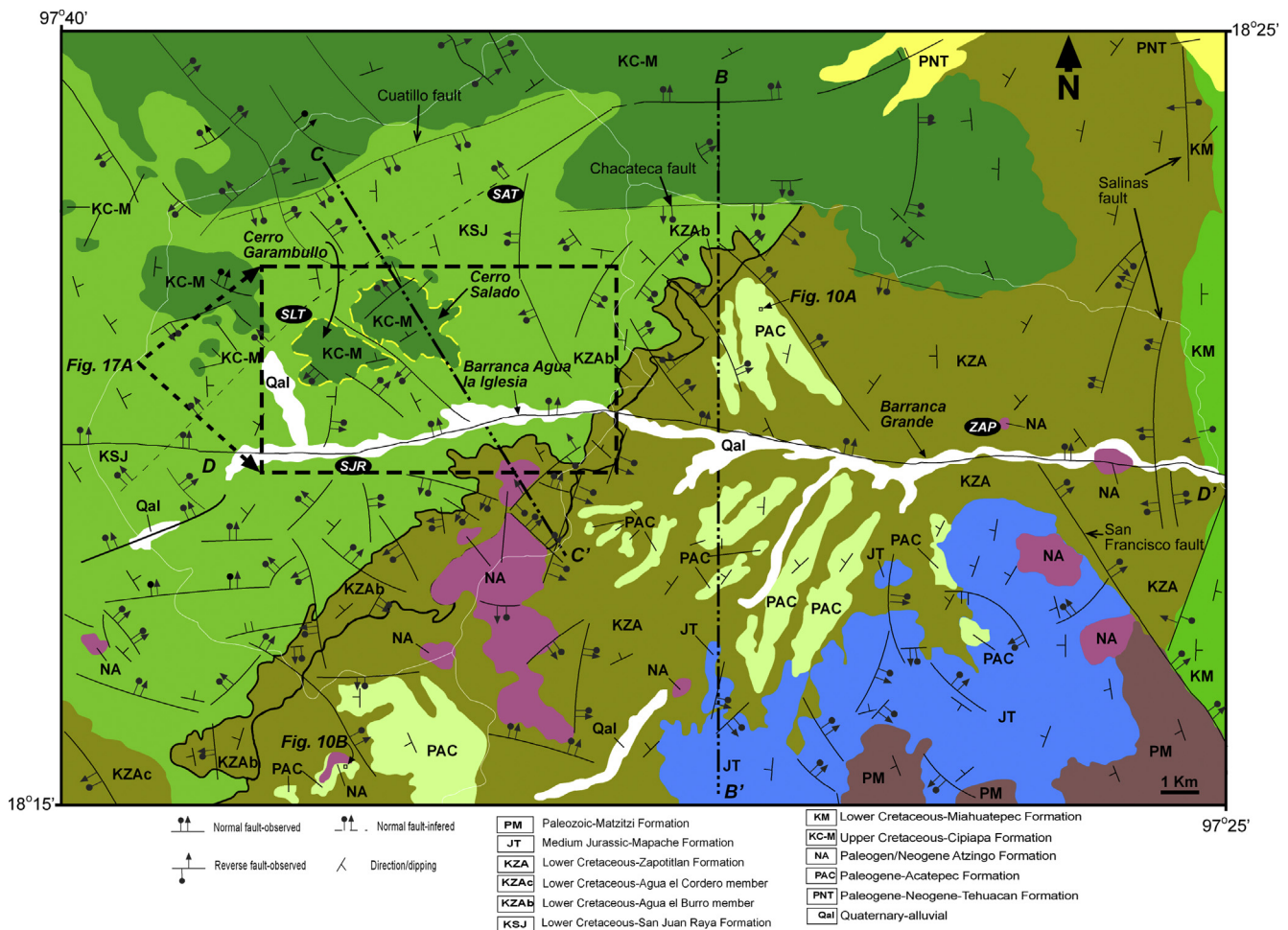
Figure 5. Geological map of the ZAPb and SJRb, modified from Buitrón and Barceló-Duarte (1980). The stratigraphic position of the lithological units for both basins are shown in Figure 6. The Zapotitlán de las Salinas (ZAP), San Juan Raya (SJR), Santa Ana Teloxtoc (SAT) and San Lucas Teteletitlán (SLT) towns are also indicated. The Cerro Salado and Cerro Garambullo tectonic klippe are outlined. Location of the B-B' (Figure 12), C-C' (Figure 14) and D-D' (Figure 13) transects and the approximate area of Figure 17A (dashed rectangle) are also indicated.
