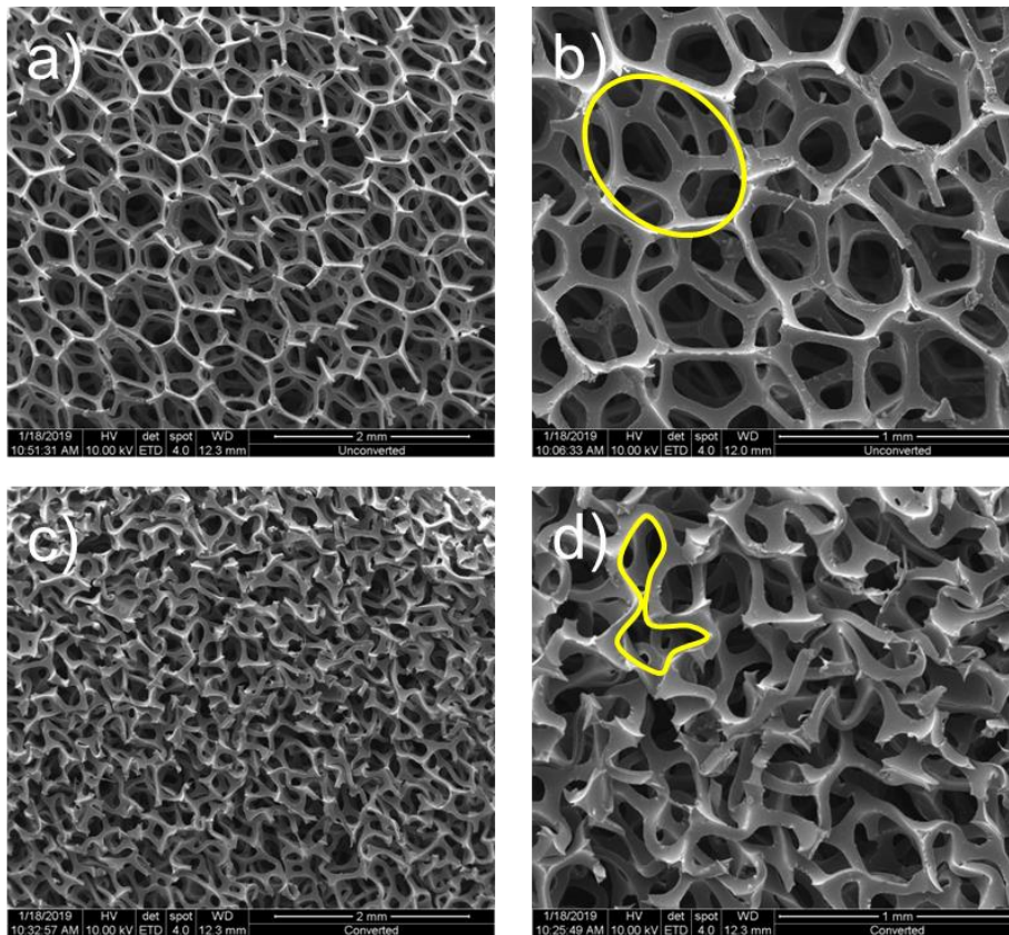
Figure 4 , SEM images of cross sections of uncompressed and tri-axially compressed polyurethane foam. a) Uncompressed foam showing pores with regular well-ordered structure (scale bar 2mm). b) Higher magnification image of uncompressed foam with example uniform pore highlighted in yellow (scale bar 1mm). c) tri-axially compressed polyurethane foam showing irregular pores with a re-entrant structure (scale bar 2mm). d) Higher magnification image of foam with example re-entrant bowtie structure highlighted in yellow (scale bar 1mm).
