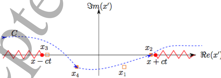
FIG. 6. The complex plane in which the integration contour C is deformed through the saddle points at x_2 and x_4 . The branch cut emanating from the branch points at x' = x \pm ct is shown in red.
