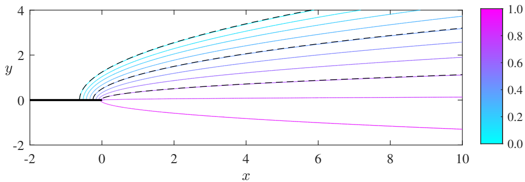
Figure 4: Contours of the steady flow depth for the case \alpha = \pi . Contours of the numerical result (continuous coloured lines) are plotted at h = 0.01, 0.1, 0.2, 0.3, 0.4, 0.5, 0.6, 0.7, 0.8, 0.9 . The thick black line represents the wall. Contours of the exact solution (5.4), plotted as dashed lines for h = 0.01, h = 0.4 and h = 0.7 show excellent agreement.
