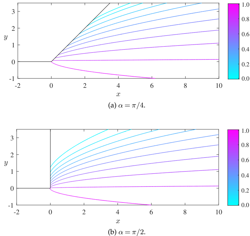
Figure 2: Contour plots of the dimensionless thickness of the steady flow, h(x, y) in a channel that expands at x=0 for two values of the opening angle, \alpha : (a) \alpha = \pi/4 and (b) \alpha = \pi/2 . The results are obtained numerically, as described in §3. Contours are plotted at h = 0.01, 0.1, 0.2, 0.3, 0.4, 0.5, 0.6, 0.7, 0.8, 0.9 .
