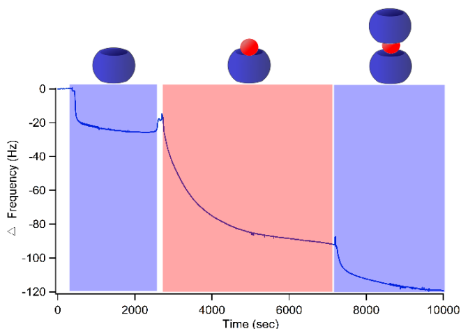
Fig. 2 Quartz Crystal Microbalance data demonstrating the layer-by-layer build up of CB[7]- \text{Fe}^{3+} nano-layers.
