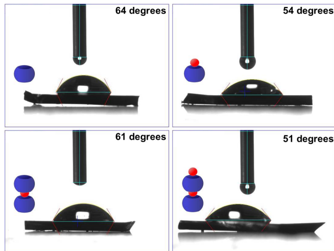
Fig. 3 Contact angle measurements highlighting the changes in hydrophobicity of a gold substrate after the layer-by-layer deposition of the CB- \text{Fe}^{3+} nanostructure.
