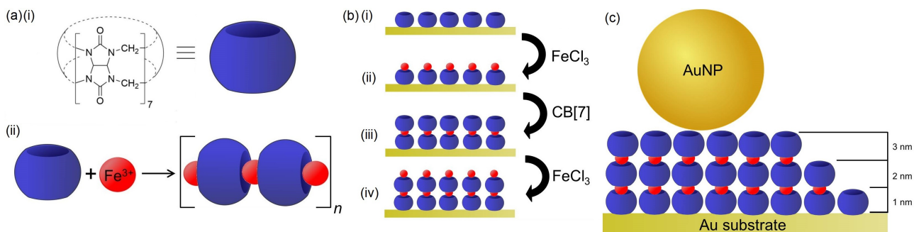
Fig. 1 (a)(i) The chemical structure of CB[7] is shown. (ii) A coordination complex forms when \text{Fe}^{3+} and CB[7] are mixed in water. (b) Schematic of the layer-by-layer process used to build up coordination complexes of CB[7] and \text{FeCl}_3 \cdot 6\text{H}_2\text{O} onto gold substrates. (c) An illustration highlighting that surface deposited CB[7]- \text{Fe}^{3+} can be used to yield well defined spacings with nanometer control in plasmonic systems consisting of a gold film and a gold nanoparticle.
