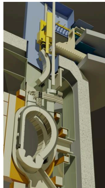
Fig. 1: Vertical port blanket extraction handling scheme
