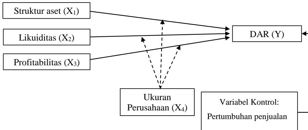
Gambar 1. Model Penelitian
