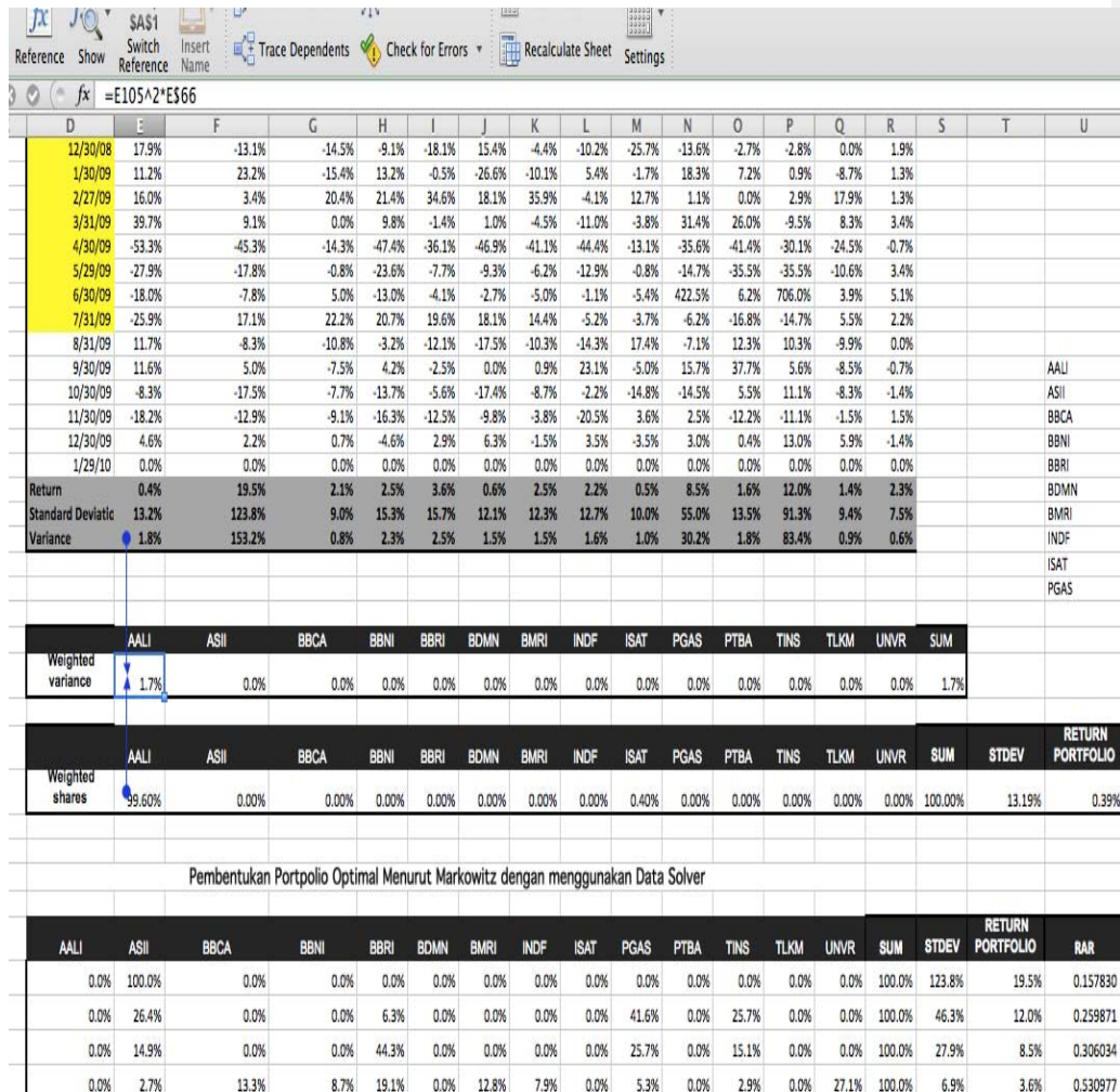
Gambar 4.1 WEIGHTED VARIANCE
