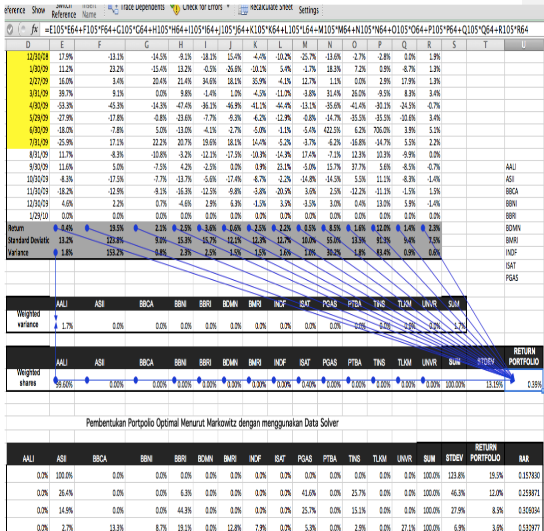
Gambar 4.2 RETURN PORTFOLIO
