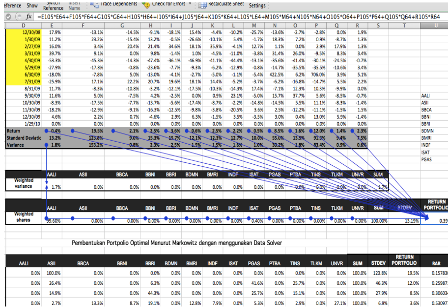
Gambar 4.2 RETURN PORTFOLIO
