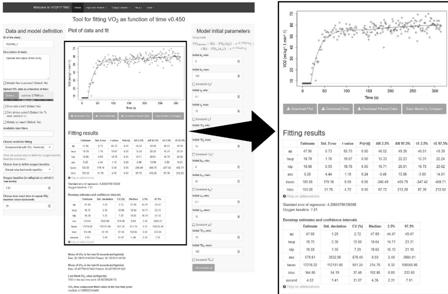
Figure 2. VO 2 FITTING home menu with an individual example of a T400 modelled VO 2 response (bi-exponential) in the middle. Data and model definition , and model initial parameters menu without any constraint for parameter estimates are presented in upper-left and right corner, respectively.
