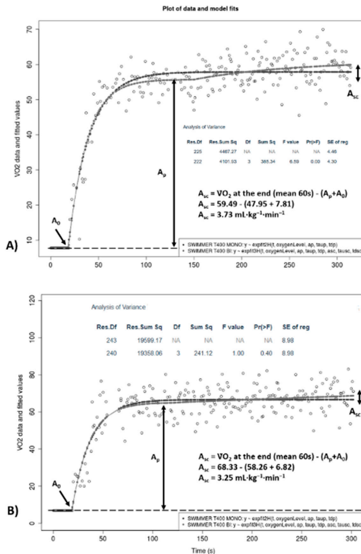
Figure 3. Examples of goodness-of-fit analysis between mono- and bi-exponential models of a typical T400 \text{VO}_2 response from two swimmers. (A) bi-exponential model being superior; (B) No difference between mono- and bi-exponential models. Shapiro–Wilk (residuals distribution) and ANOVA F-test (with respective residuals sum of the squared from the differences between both models) detailed on the top of both graphics. * Res.Df: residual degree of freedom; Res.Sum Sq: residual sum of square; Df: degree of freedom; Sum Sq: sum of square; F value: for testing the hypothesis that the group means for that effect are equal; Pr(>F): the significance probability value associated with the F Value; SE of reg: standard error of regression.
