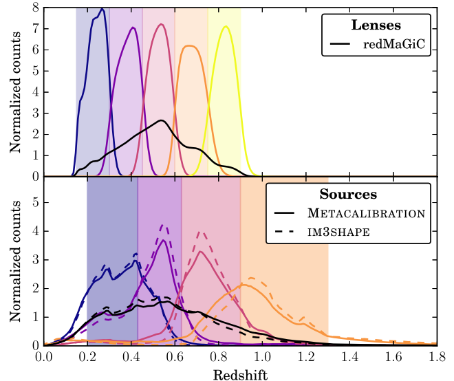
FIG. 1. Estimated redshift distributions of the lens and source galaxies used in the Y1 analysis. The shaded vertical regions define the bins: galaxies are placed in the bin spanning their mean photo- z estimate. We show both the redshift distributions of galaxies in each bin (colored lines) and their overall redshift distributions (black lines). Note that source galaxies were chosen via two different pipelines IM3SHAPE and METACALIBRATION, so their redshift distributions and total numbers differ (solid vs dashed lines).
