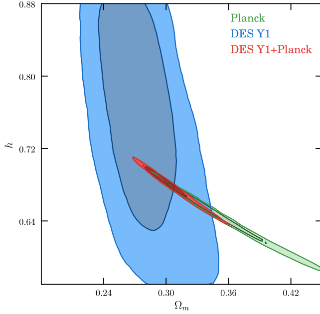
FIG. 12. \Lambda CDM constraints from Planck with no lensing (green), DES Y1 (blue) and the two combined (red) in the \Omega_m - h plane. The positions of the acoustic peaks in the CMB constrain \Omega_m h^3 extremely well, and the DES determination of \Omega_m breaks the degeneracy, leading to a larger value of h than inferred from Planck only (see Table II).
