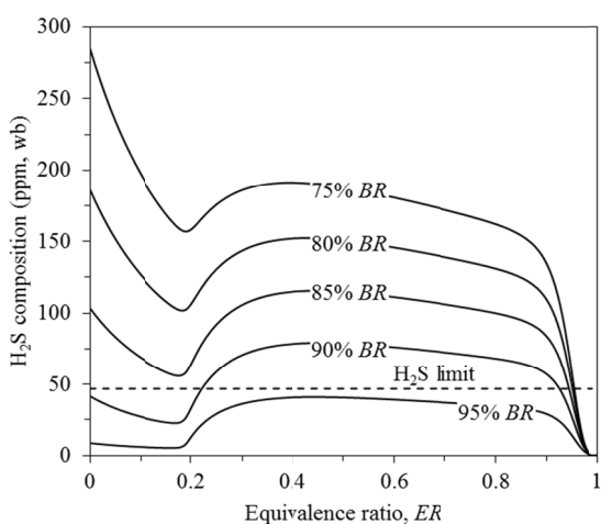
Figure 8: H_2S contents for dry coal-wood co-gasification in the ranges 0 \leq ER \leq 1 and 75 \leq BR \leq 95\% at 1000^\circ C . Dashed line (---) indicates the H_2S limit for cogeneration.
