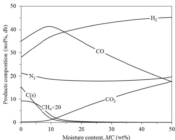
Figure 4: Composition of gaseous products and non-converted carbon for coal gasification at ER = 0.1 and 1000 °C in the range 0 \leq MC \leq 50\% .
