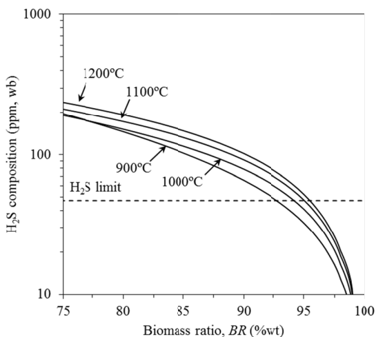
Figure 7: H_2S content for dry coal-wood co-gasification in the range of 75 \leq BR \leq 100\% and 900 \leq T \leq 1200^\circ C at ER = 0.4 . Dashed line (---) indicates the H_2S limit for cogeneration.
