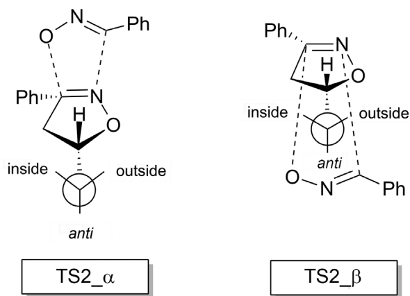
Figure 1. Transition structures (schematically presented) obtained for the second cycloaddition. The 1,3-dipole approaches by the sterically less hindered face (on the right) and 1,3-dipole approaches by the sterically more hindered face (on the left).
