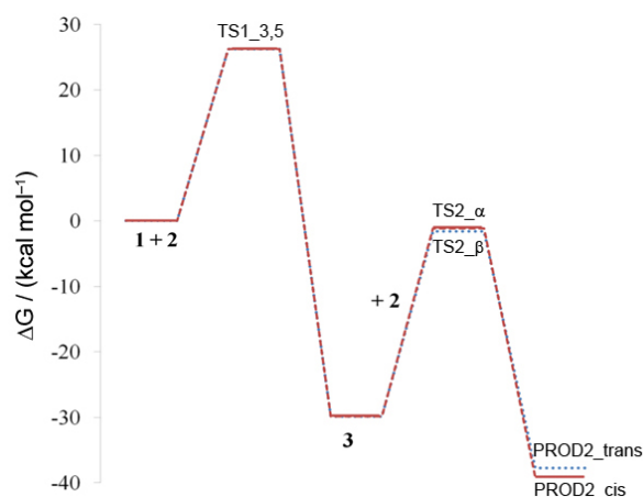
Figure 5. Free energy profile (in kcal mol -1 ) for the two subsequent cycloadditions in the gas phase, using PBE1PBE as functional. The energies of TS1 and PROD1 are related to 1 + 2 . The energies of TS2 and PROD2 are related to 3 + 2 .
