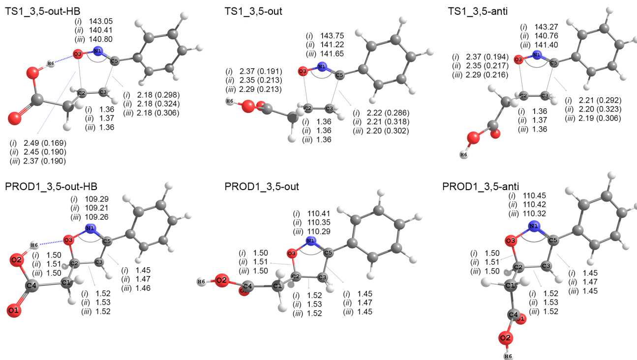
Figure 2. Geometries of lower energy transition structures for the first cycloaddition (TS1) and corresponding products obtained in the gas phase, showing the new bond lengths formed and respective Wiberg bond index (in parentheses), the angles between C 5 –N 1 –O 3 and the C 2 –C 3 bond lengths. The functionals used are: (i) PBE1PBE, (ii) B3LYP and (iii) CAM-B3LYP. All bond lengths are in Å and angles in degrees.
