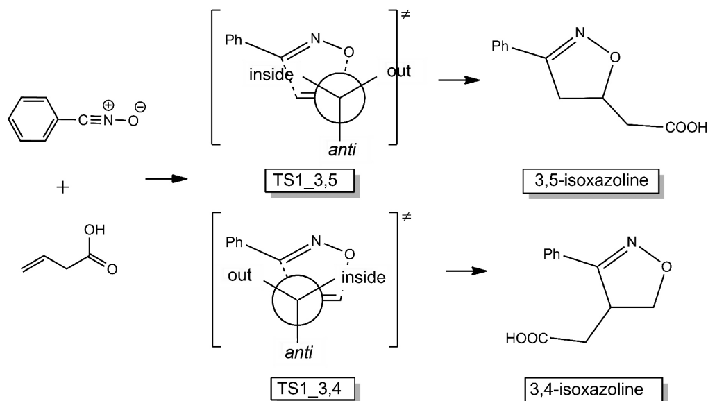
Scheme 2. Reaction scheme for the two regioisomers. Highlighted are the three possible positions for the substituent in the \alpha -carbon in transition structures.
