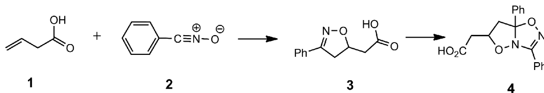
Scheme 1. [3 + 2] 1,3-Dipolar cycloaddition reaction between vinylacetic acid ( 1 ) and nitrile oxide ( 2 ) yields the cycloadduct ( 3 ) and afterwards the 2:1 cycloadduct ( 4 ).
