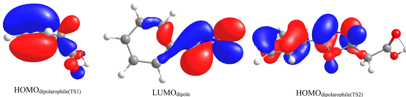
Figure 3. Frontier molecular orbitals (in the TS geometry) involved in the two cycloaddition reactions.
