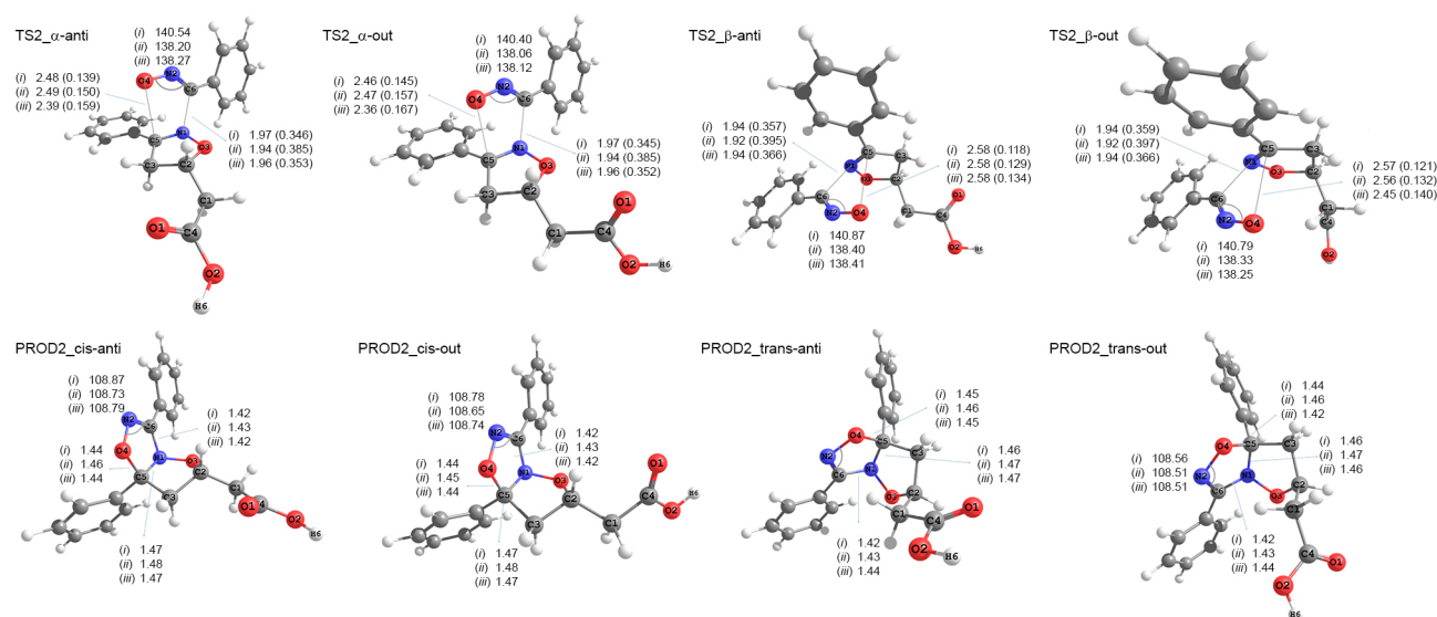
Figure 4. Geometries of lower energy transition structures for the second cycloaddition (TS2) and corresponding products obtained in the gas phase, showing the new bond lengths formed and respective Wiberg indices (in parentheses), and angles between C 5 -N 1 -O 3 . The functionals used are: (i) PBE1PBE, (ii) B3LYP and (iii) CAM-B3LYP. All bond lengths are in Å and angles in degrees
