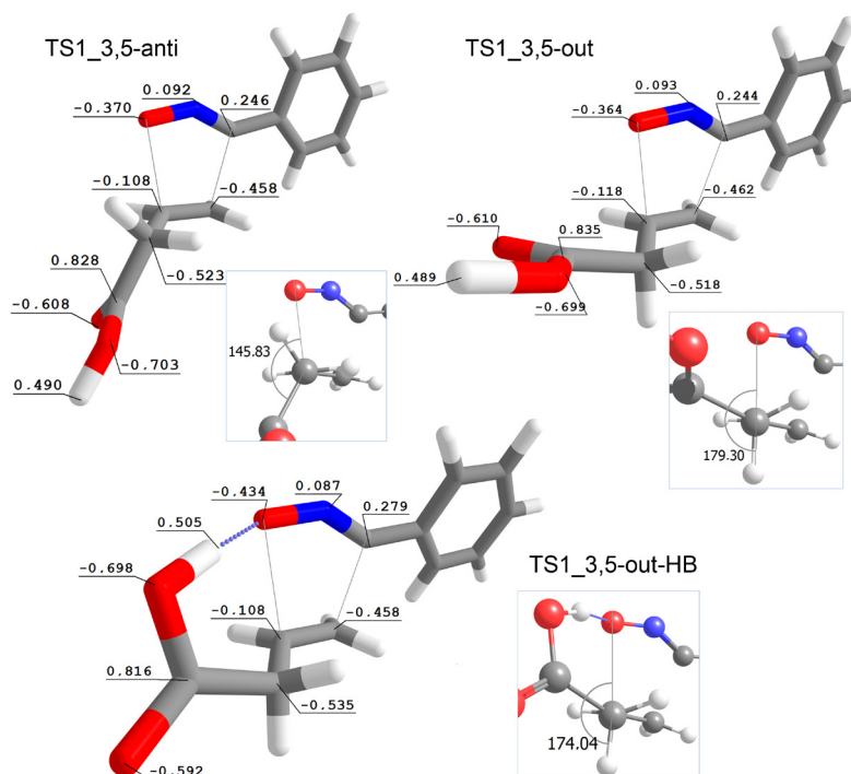
Figure 6. Natural atomic charges obtained for the TS1 calculated at B3LYP/6-311+G(2d,p) level of theory, in the gas phase. Dihedral angles between the oxygen of 1,3-dipole and the group at anti position are highlighted.
