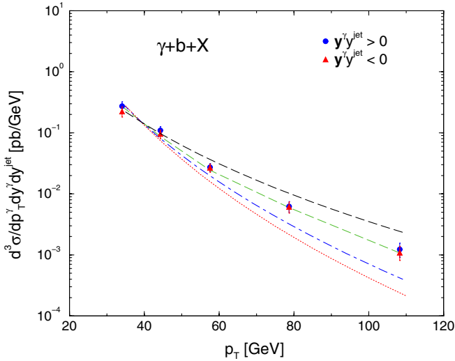
FIG. 2 (color online). The \gamma + b + X differential cross section as a function of p_T^\gamma . Experimental data from the D0 Collaboration [8] (only systematic errors are presented).
