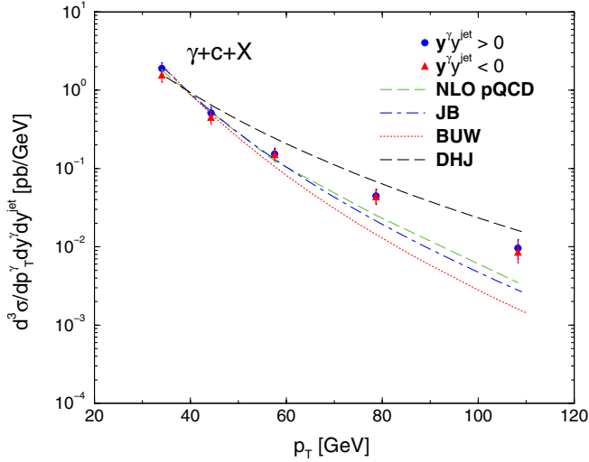
FIG. 1 (color online). The \gamma + c + X differential cross section as a function of p_T^\gamma . Experimental data from the D0 Collaboration [8] (only systematic errors are presented).
