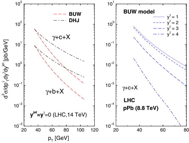
FIG. 3 (color online). The \gamma + Q + X differential cross section at LHC regime. (Left) proton-proton cross sections at central jet/photon rapidities as a function of p_{\perp}^{\gamma} at \sqrt{s} = 14 TeV. (Right) proton-lead (pPb) cross section for charm plus photon for fixed photon rapidities y^{\gamma} = 1, 2, 3, 4 at \sqrt{s} = 8.8 TeV.
