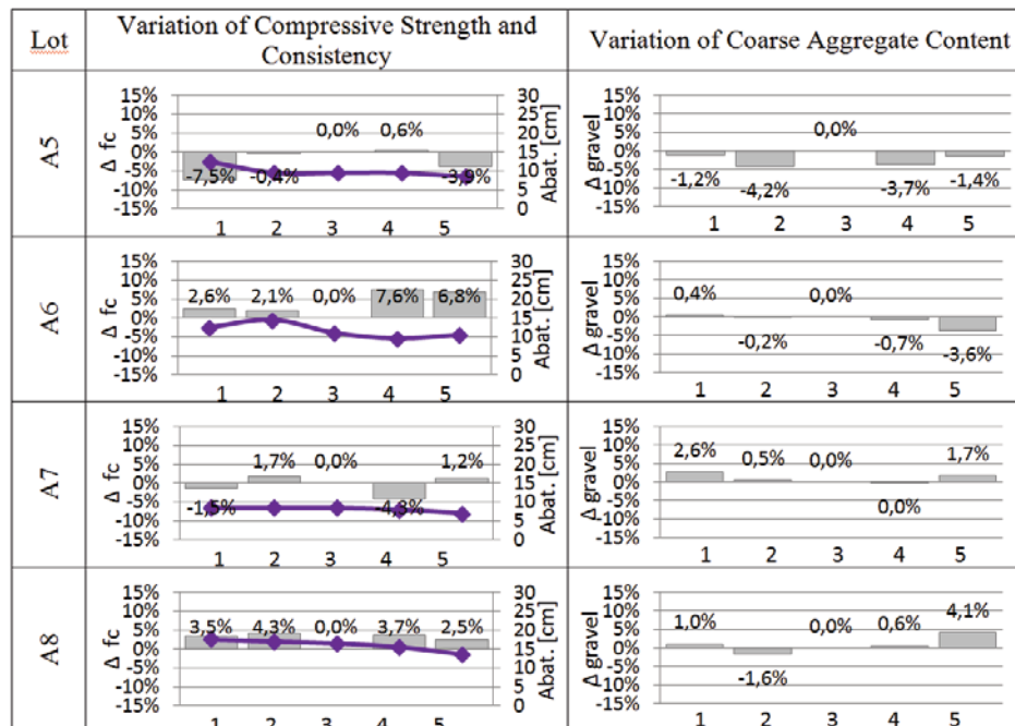
Figure 3 – Profile of variations in compressive strength, consistency and coarse aggregate content - lots 5 to 8
