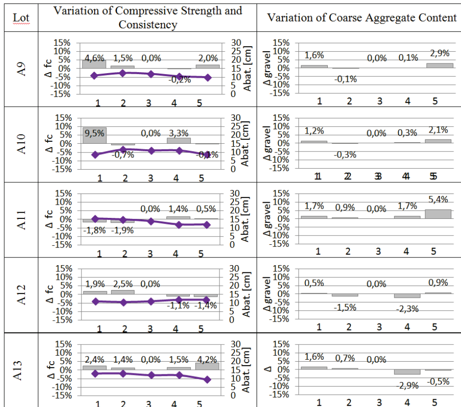
Figure 4 – Profile of variations in compressive strength, consistency and coarse aggregate content - lots 9 to 13
