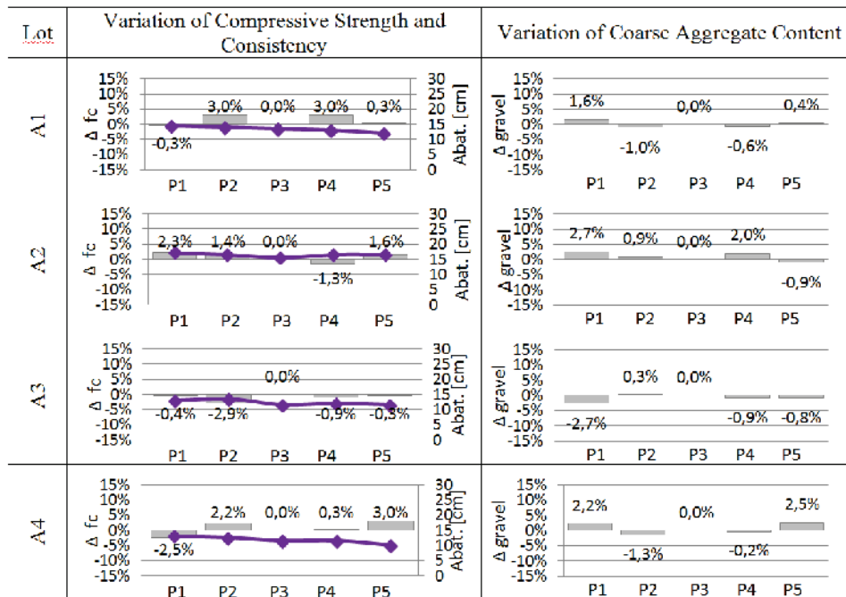
Figure 2 – Profile of variations in compressive strength, consistency and coarse aggregate content – lots 1 to 4
