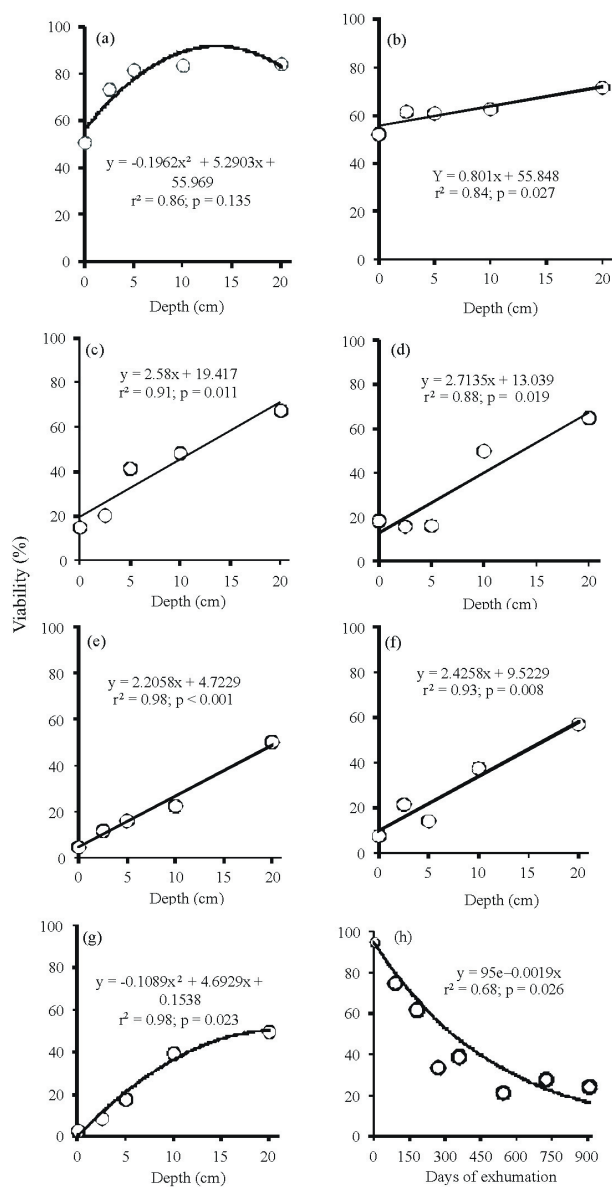
Each dot represents means of: equations (a); (b); (c) and (d) six observations; equation (e) eight; equation (f) ten; (g) twelve; equation (h) derived from exhumation seven.
