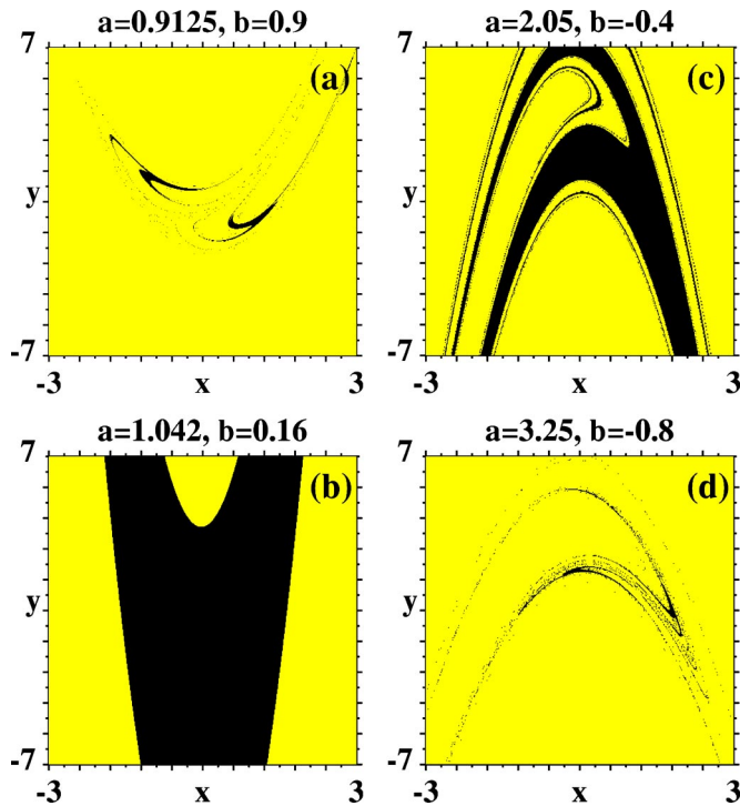
FIG. 2. (Color online) Illustrative basins computed for four different set of parameters along the 2 \rightarrow 4 bifurcation line, defined by Eq. (3): (a) (a, b) = (0.9125, 0.9) ; (b) (1.042, 0.16) ; (c) (2.05, -0.4) ; (d) (3.25, -0.8) . The gray shading indicates the basin of -\infty , black gives the basin of the periodic motion.
