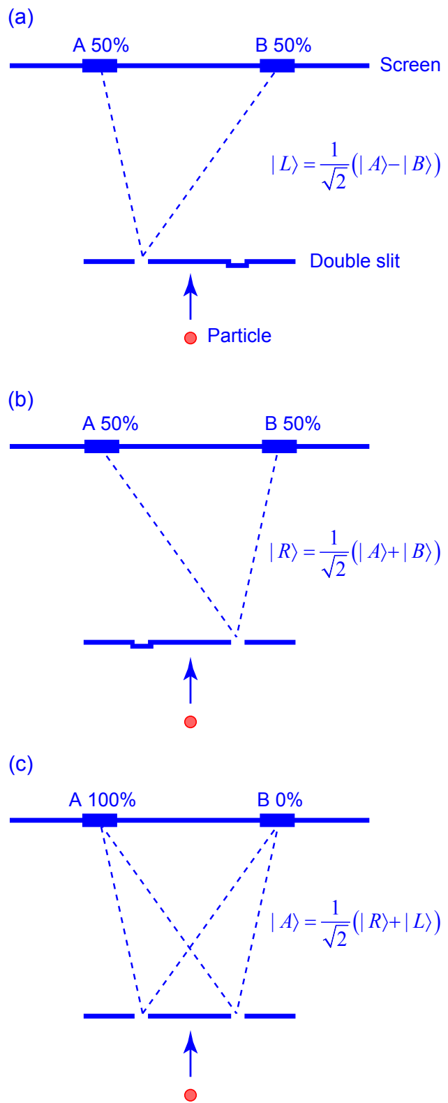
Figure 1: Hypothetical experiment with only two possible outcomes ( A and B ). Panel (a) only the left slit is open. Panel (b) only the right slit is open. Note, each slit is not a simple hole but acts as a filter which projects the particle either to a trajectory with endpoint A or to a trajectory with endpoint B . Panel (c) shows the experiment with both slits open: interference takes place and all particles hit the screen in A .
