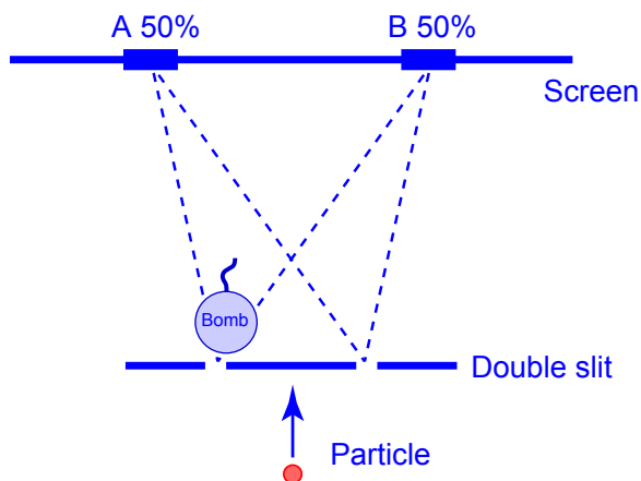
Figure 2: Variant of the Elitzur–Vaidman experiment: a bomb is placed just after the left slit.
