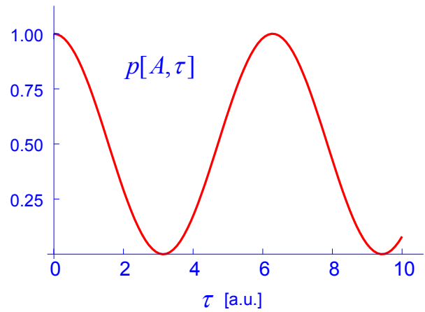
Figure 5: Quantity p[A, \tau] as function of \tau in the case of entanglement with an idler state according to Eq. 41.
