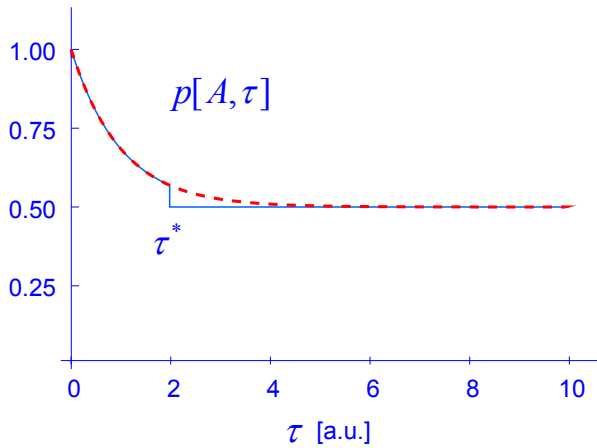
Figure 4: The quantity p[A, \tau] is plotted as function of \tau . The dashed line represents the prediction of the unitary evolution of Eq. 25. The solid line represents the prediction of the collapse hypothesis of Eq. 35: if the detection of the screen takes place for \tau larger than the critical value \tau^* , the state has collapsed to either A or B, therefore p[A, \tau > \tau^*] = 1/2 . Note, we use arbitrary units. The choice of \tau^* is also arbitrary and serves to visualize the effect (it is expected to be much larger in reality).
