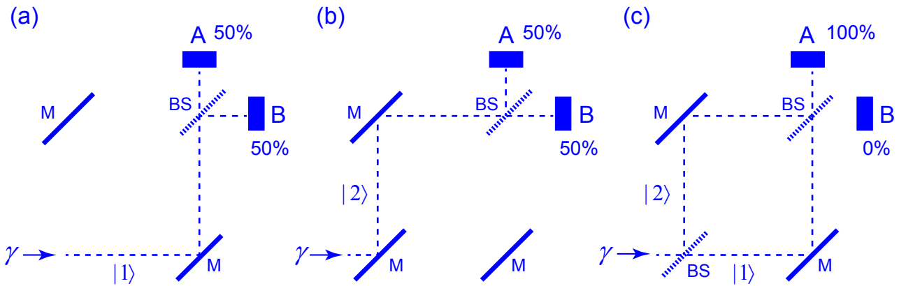
Figure 3: The Mach–Zehnder interferometer. In analogy with the setup shown in Fig. 1, the case (a) corresponds to only the left slit open, (b) to only the right slit open, (c) to both slits open. The interferometer paths are adjusted so that constructive interference occurs at detector A and destructive interference occurs at detector B. M, mirror; BS, beam splitter; \gamma , photon.
