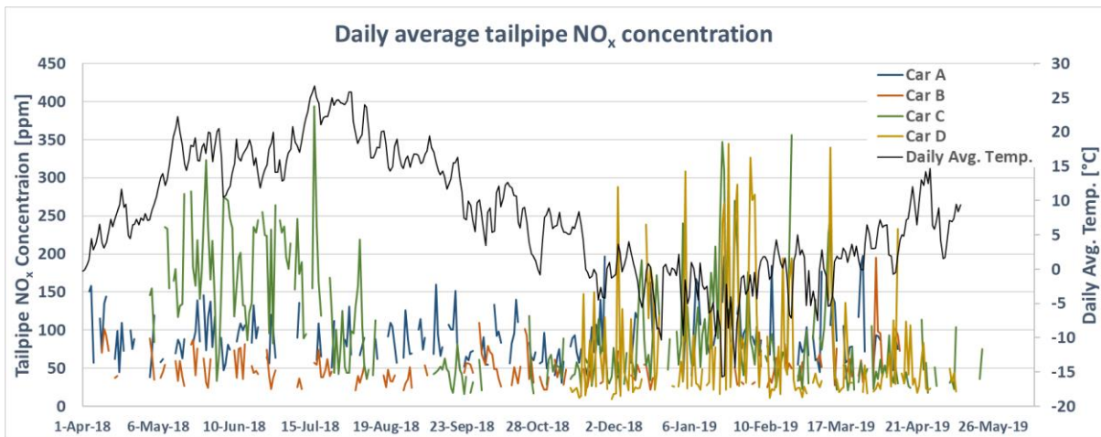
Figure 28: Daily average NO x concentration during the project period.
