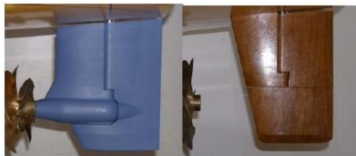
Figure 3.1.3.3.- Comparison of areas and rudder axis location
