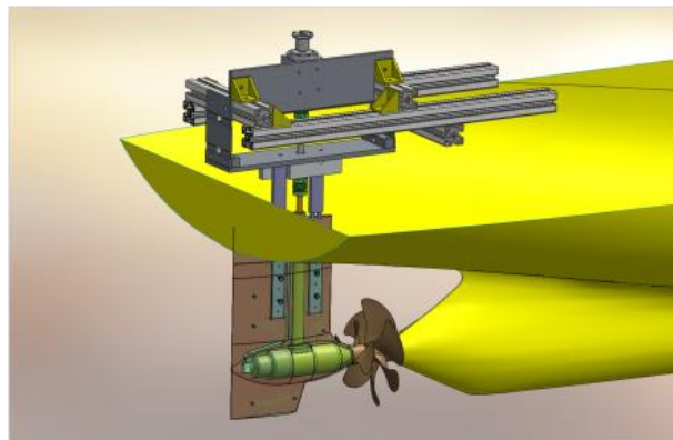
Fig. 3.1.1.1.- Arrangement for self propulsion tests.
