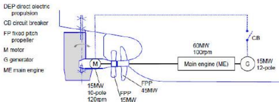
Figure 3.1.3.1.- Rudder-Pod system.
