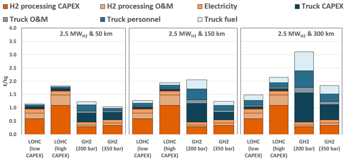
Figure 26. Detailed cost breakdowns for 2.5 MW hydrogen demand cases (50, 150 and 300 km). H 2 processing includes compression, hydrogenation, dehydrogenation and related site costs (piping, buildings, engineering) but not purification.
