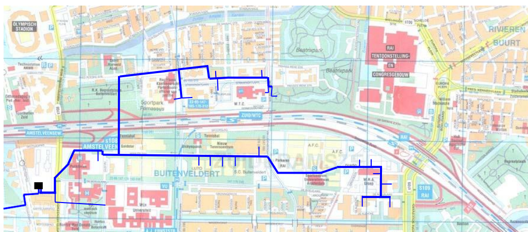
Figure 11: The DC system in Zuidas, Amsterdam
