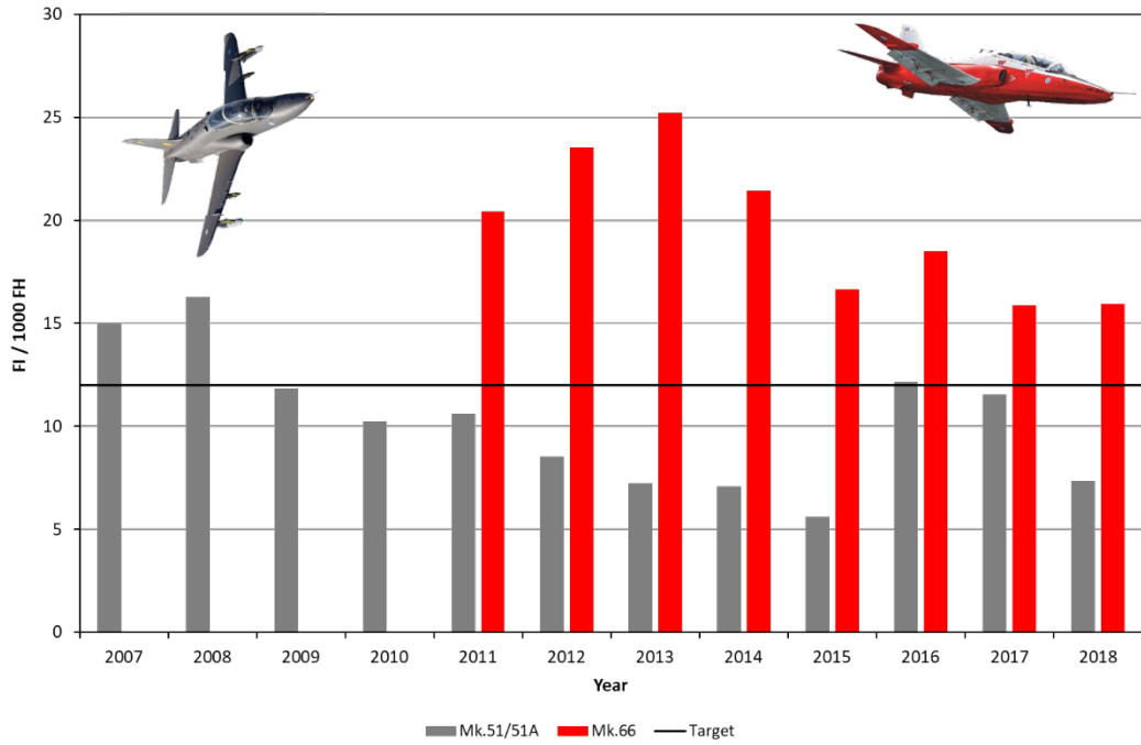
Figure 8: Annual Fatigue Index (FI) development of the FINAF Hawk aircraft (Mk.51/51A in grey; Mk.66 in red) in the end of 2018. The annual target, average of all the types, is 12 FI/1000 FH. Figure courtesy of the FINAF.
