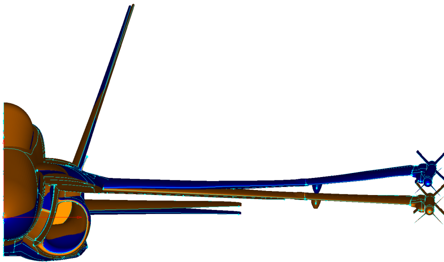
Figure 17: Surface grid shape of the Hornet in its nominal form (orange) and with converged static aeroelastic deformations (blue) in a symmetric steady pull-up case at the limit load factor. Figure courtesy of Patria Aviation.
