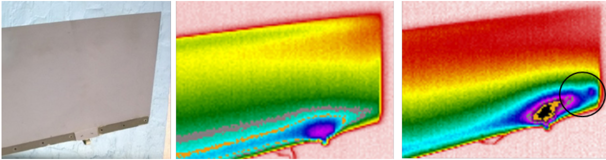
Figure 63: An overview of the rudder thermography inspections. Left: Actual rudder. Middle: Normal thermal pattern image i.e. no moisture ingress (LYK0059 (U22-2803)). Right: Abnormal thermal pattern image, which was verified by analysis as a positive finding of moisture ingress (LYK0132 (U22-2940)). Figure courtesy of VTT.
