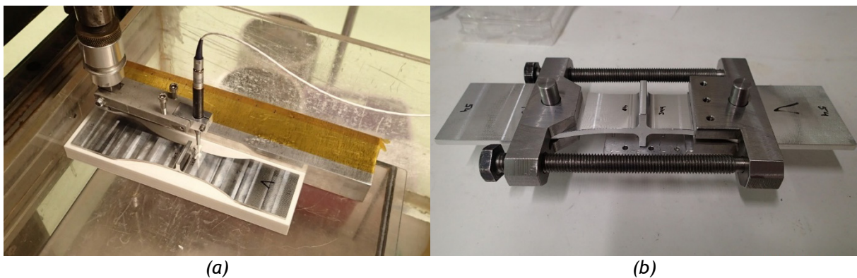
Figure 32: Automated Eddy Current inspections (subfigure a), static loading frame for SEM analysis (subfigure b). Figure courtesy of VTT.
