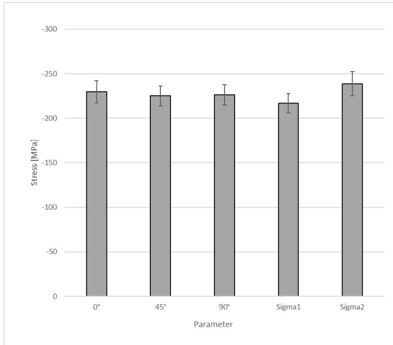
Figure 38: The average residual stresses of 12 test specimens in 3 distinctive directions (0°, 45°, 90°), and max/min principal directions (Sigma1, Sigma2) from the X-Ray Diffraction measurements prior to the fatigue tests. Figure courtesy of Aalto University.
