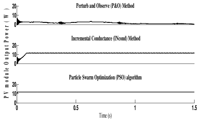
Fig. 12 The PV module output power (w) simulated with the MATLAB model at 200kw/m 2 , 25°C.
