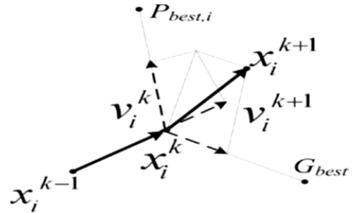
Fig. 7. Movement of a PSO particle.
