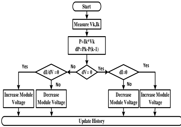
Fig. 5 Flowchart of P&O algorithm.
