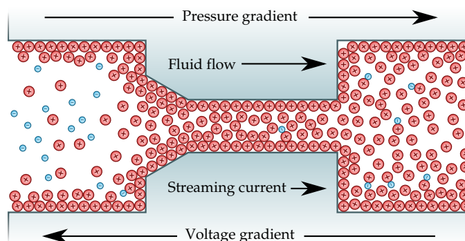
Fig. 1. Conceptualised rendering of the cross section of a streaming cell. Positive ions are being forced through the cavity by the application of pressure.
