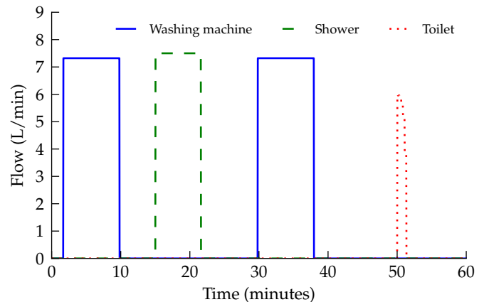
Fig. 6. Sample profile showing constructed instances of washing machine use, a shower and a toilet flush. Washing machine usage is broken into two parts corresponding to a wash and rinse cycle.
