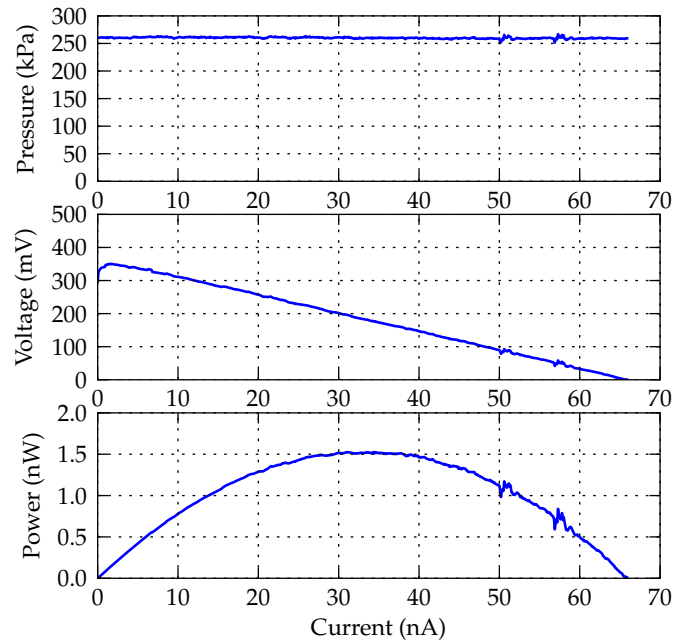
Fig. 5. Streaming cell output voltage as a function of drawn current with constant pressure. The cell's calculated output power appears in the lower plot with a peak at approximately 33.5 nA.
