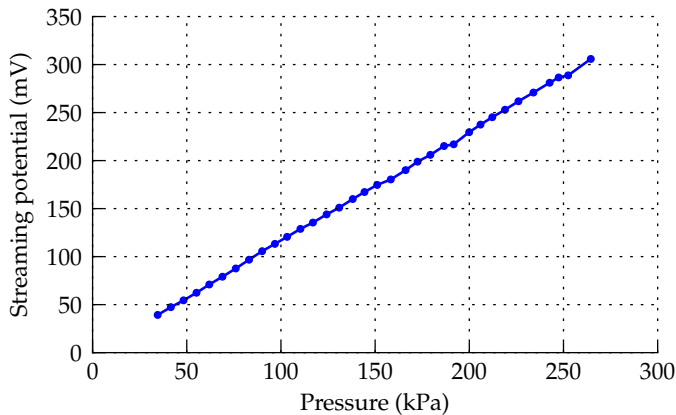
Fig. 4. Measured voltage developed across the 52 \mu\text{m} streaming cell as a function of the differential pressure across the cell.
