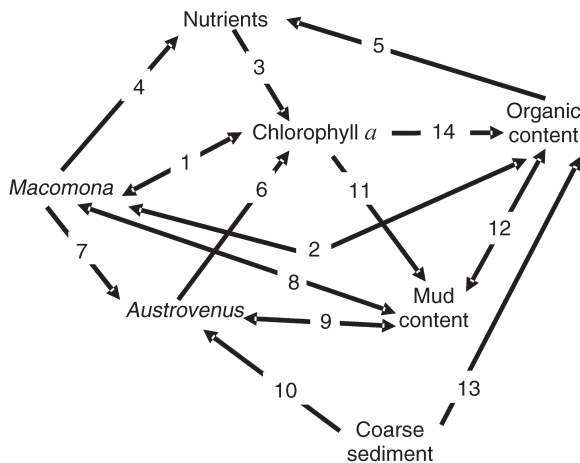
FIG. 1. Conceptual diagram of the potential interaction network linking infaunal bivalves (here marine species Macomona liliana and Austrovenus stutchburyi in New Zealand) to benthic chlorophyll a and sediment characteristics. (1) Grazing by deposit-feeding Macomona affects microphytobenthos (MPB, represented as chlorophyll a ), and MPB has a positive relationship with Macomona density. (2) Sediment organic content increases food resources for Macomona . (3) MPB are highly productive and exploit nutrients remineralized in sediments. (4) Macomona affect pore water nutrient concentrations directly and (2, 5) indirectly. (6) Austrovenus has a positive effect on MPB. (7) Large Macomona and small Austrovenus interact negatively. (8, 9) Sediment mud content negatively affects density of both bivalve species; high densities of both species can increase fine-sediment erosion. (10) In coarse sediments, Austrovenus density increases. (11) MPB and mud content have a positive relationship, (8, 9) mediated by resident macrofauna. (12) Mud and sediment organic content are tightly correlated and (13) coarse sediments influence sediment organic content by increasing permeability and decay. (14) Degrading MPB also contributes to sediment organic matter, which (5) is positively correlated with nutrient concentration in pore water through microbial degradation. See Methods for further details and references.
