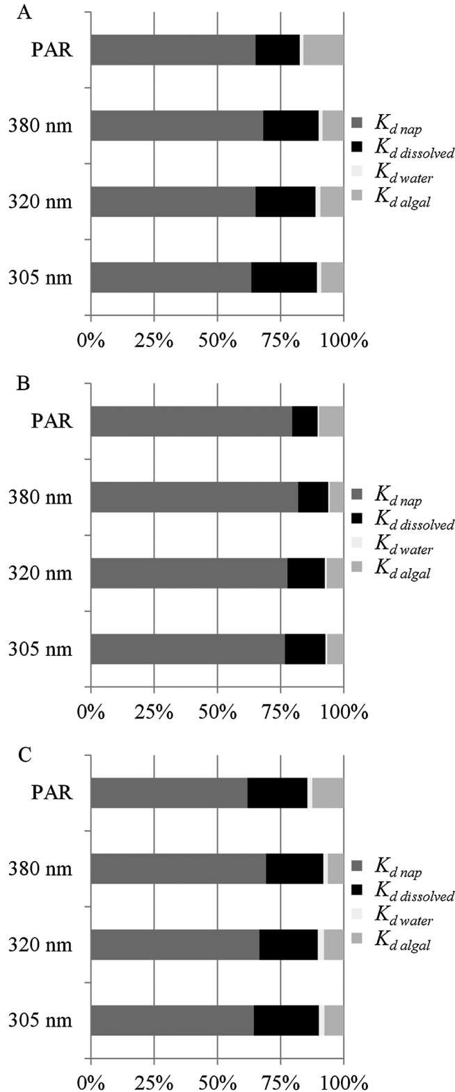
Figure 4. Percentages of the total diffuse attenuation coefficients from nonalgal particulates ( K_{d\text{ nap}} ), dissolved substances ( K_{d\text{ CDOM}} ), water ( K_{d\text{ water}} ), and phytoplankton ( K_{d\text{ algal}} ) with turbidity-specific attenuation coefficients derived in all lakes and applied to all lakes (A), derived from New Zealand lakes and applied to New Zealand lakes (B), and derived from Canadian Rockies lakes and applied to Canadian Rockies lakes (C). Glacial flour is assumed to be the dominant contributor to K_{d\text{ nap}} .
