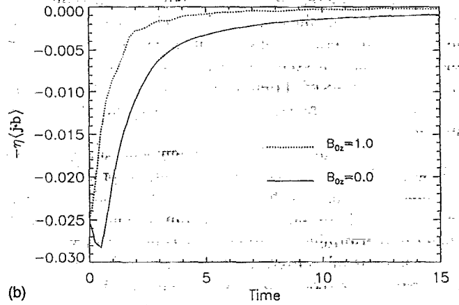
FIG. 13. In (a) the time history of the nonlinear H_m decay term [see Eq. (22)] -\mathbf{B}_0\cdot\langle\mathbf{v}\times\mathbf{b}\rangle is compared for two 32^3 simulations with identical initial conditions, and a mean magnetic field with magnitude B_0=1 . The dotted curve is the time history for a resistive simulation, and the solid curve is the time history for a simulation with a mean magnetic field with magnitude B_0=1 , and the solid curve is the time history for a resistive simulation with no mean magnetic field.
