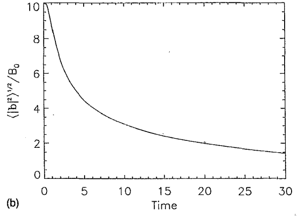
FIG. 15. Time history of the parameter \sqrt{\langle |\mathbf{b}|^2 \rangle} / B_0 for two dissipative simulations, one with high cross-helicity H_c (a) and one with low H_c (b).
