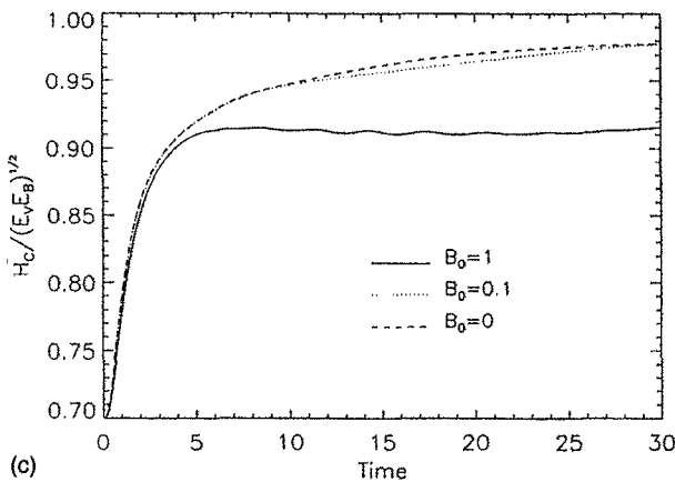
FIG. 16. Comparison of time histories of (a) H_m/E_b , (b) E_v/E_b , and (c) H_c/\sqrt{E_v E_b} , as the magnitude of the mean magnetic field B_0 is varied for three 32^3 dissipative simulations with a high cross-helicity initial condition.
