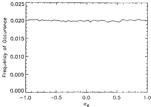
FIG. 10. Frequency of the occurrence of values of \sigma_m(\mathbf{k})=kH_m(\mathbf{k})/E_b(\mathbf{k}) computed from absolute equilibrium \mathbf{b}(\mathbf{k}) distribution. Compare with Fig. 7, which was obtained from an ideal simulation. It should also be noted that this curve is independent of the number Fourier modes M .
