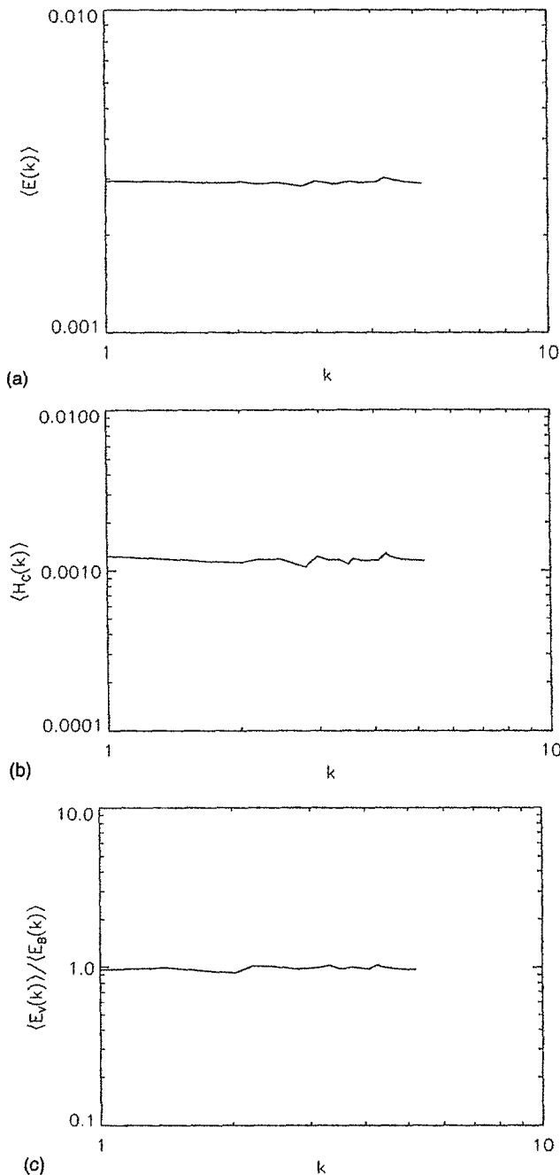
FIG. 9. Long time averages of the (a) total energy spectrum \langle E(\mathbf{k}) \rangle , (b) cross-helicity spectrum \langle H_c(\mathbf{k}) \rangle , and (c) the ratio of time-averaged kinetic energy to time-averaged magnetic energy \langle E_v(\mathbf{k}) \rangle / \langle E_b(\mathbf{k}) \rangle . These curves were obtained from averaging samples taken from the 8^3 simulation, which was integrated out to 1200 eddy turnover times.
