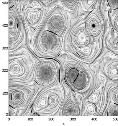
FIGURE 2. A contour map of field lines with superposed gray-shade plot of electric current density, from 2D MHD simulation. Strong current regions (very dark and very light regions) are frequently found between adjacent magnetic flux tubes, inducing a cellular structure. This feature is very clear in 2D and is present but more complex in 3D simulations. These current sheets appear as tangential discontinuities in the data samples, as in Fig. 1. It seems reasonable to suppose that a similar cellularization and origin of discontinuities might take place in the solar wind. Single spacecraft data cannot provide an unambiguous direct answer to this question.
