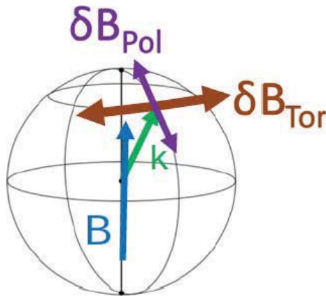
FIGURE 1. Orientation of the Tor(\mathbf{k}) and Pol(\mathbf{k}) fluctuations of with respect to \mathbf{k} and the local mean field \mathbf{B} .
