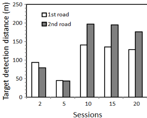
Figure 3: Vehicle detection distances
