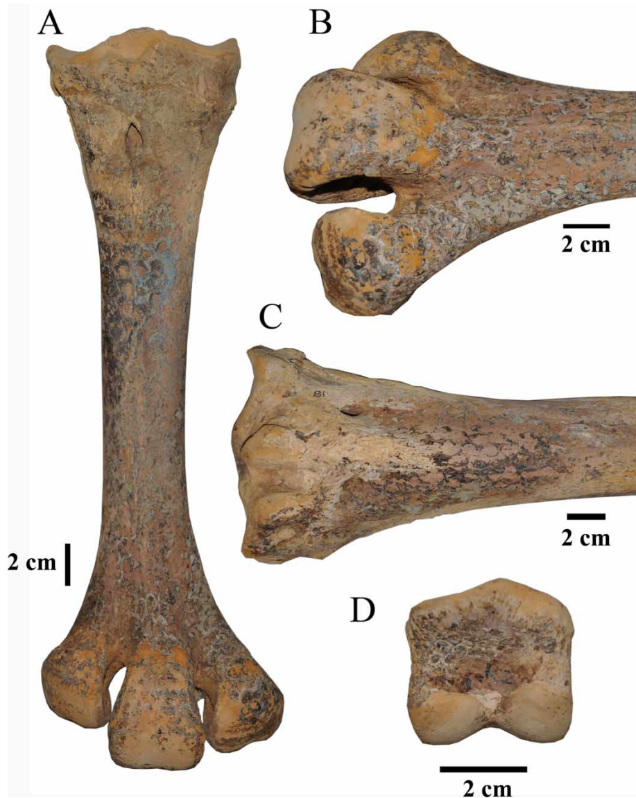
Figure 2 South Island giant moa ( Dinornis robustus Owen, 1846) with mineralised skin impressions, Ashley River, Canterbury (CMC SB1). A , Right tarsometatarsus. B , Close up of distal right tarsometatarsus. C , Ventral side of proximal right tarsometatarsus. D , Underside of phalange. The blue crystalline substance is probably the iron phosphate mineral vivianite.
