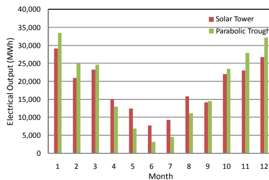
Figure 5: Output from solar power plant near Nelson
