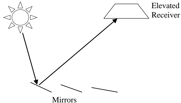
Figure 2: Schematic representation of a linear Fresnel reflector
