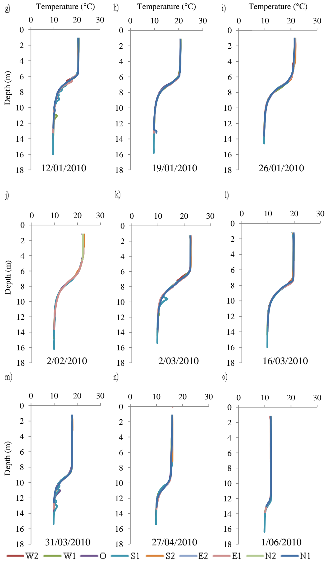
Figures 3.5g-o: Temperature profiles for all stations from 12 January 2010 – 01 June 2010.
