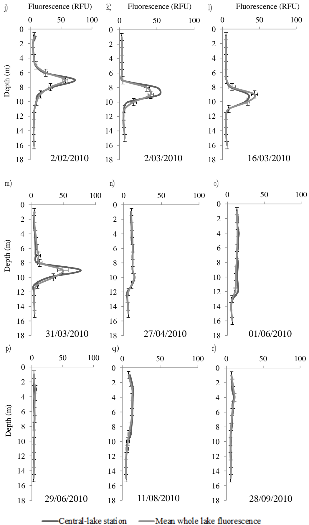
Figures 3.11j-r: Fluorescence (RFU) at central station and whole lake mean fluorescence with standard error from 02 February 2010 to 28 September 2010.
