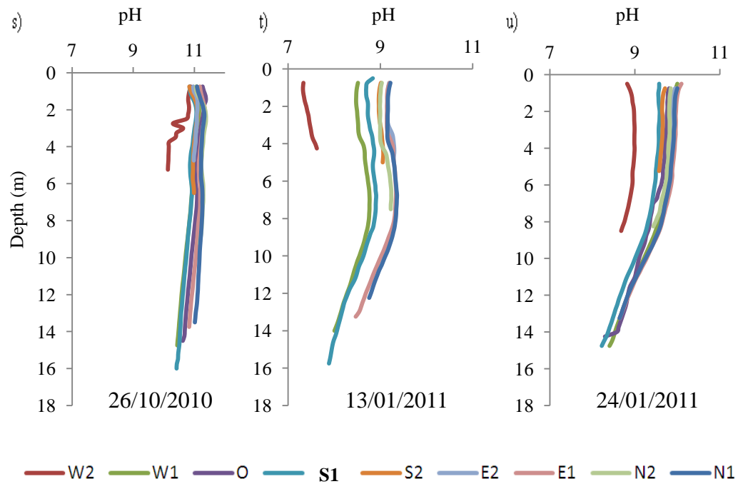
Figures 3.8s-u: pH for all stations from 26 October 2010 to 24 January 2011.
