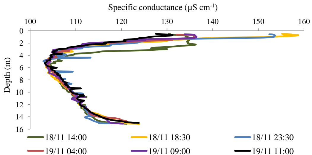
Figure 4.4: Specific conductance on 18-19 November 2010. Date and time (h) of each profile are given in inset.
