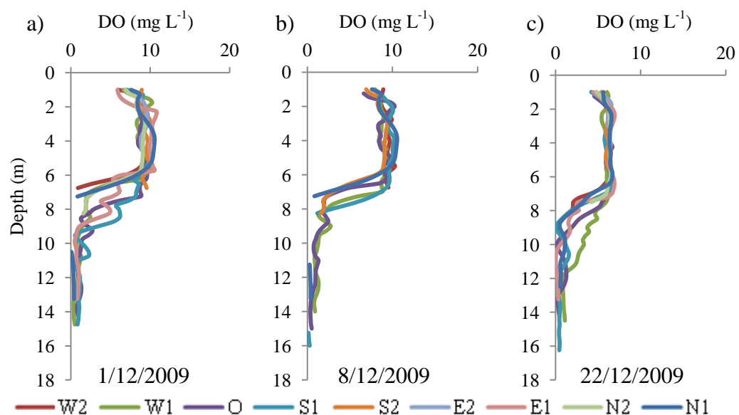
Figures 3.7a-c: Dissolved oxygen profiles for all stations from 12 December 2009 to 22 December 2009.
