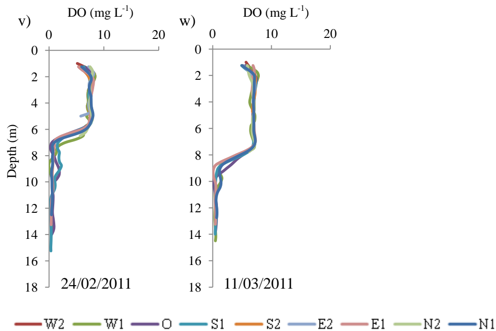
Figures 3.7v-w: Dissolved oxygen profiles for all stations from 24 February 2011 to 11 March 2011.
