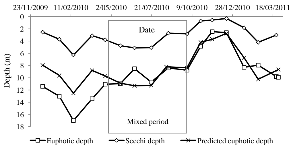
Figure 9.1: Euphotic depth, Secchi depth and predicted euphotic depth (e.g., Tilzer, 1988) from 17 December 2009 to 29 March 2011
