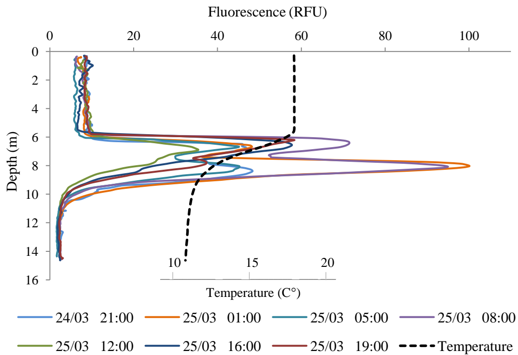
Figure 4.10: Chlorophyll fluorescence and mean temperature profile on 24-25 March 2011. Date and time (h) of each profile are given in inset.
