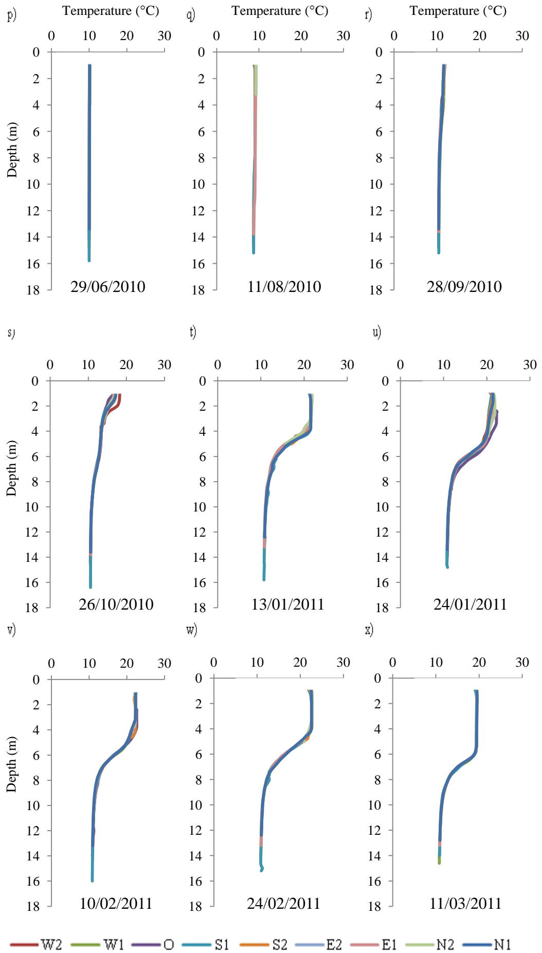
Figures 3.5p-x: Temperature profiles for all stations from 29 June 2010 – 11 March 2011.
