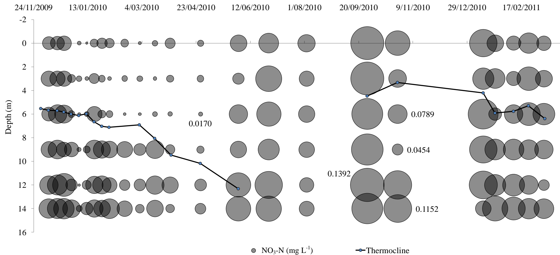
Figure 3.10b: Concentrations of \text{NO}_3\text{-N} at 0, 3, 6, 9, 12 and 14 m depth in samples taken from 08 December 2009 - 11 March 2011, and thermocline depth. Reference values are given next to several sample points ( \text{mg L}^{-1} ).
