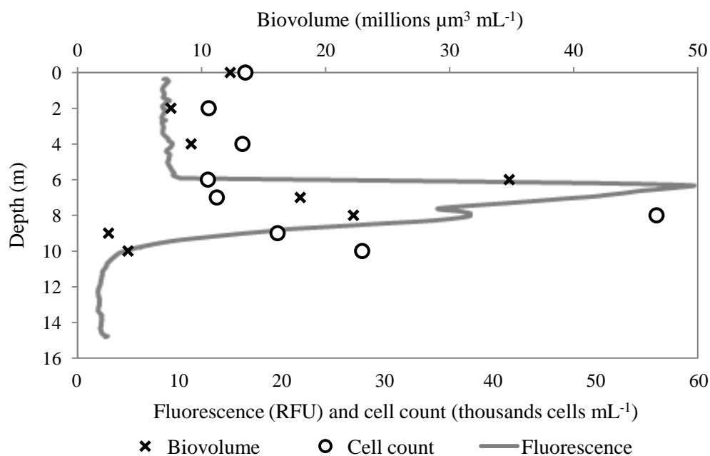
Figure 4.11: Chlorophyll fluorescence in relative units, total cell concentrations and phytoplankton biovolumes at 19:00 h on 25 March 2011
