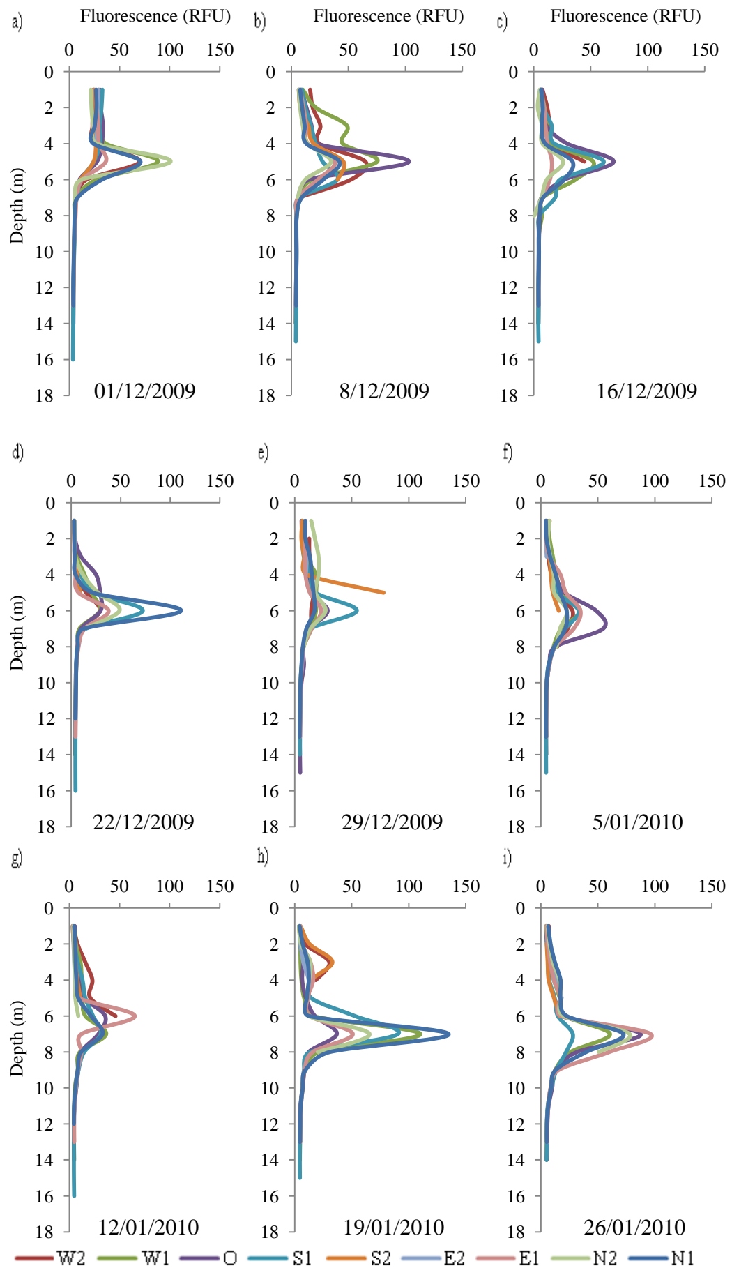
Figures 3.6a-i: Fluorescence profiles for all stations from 01 December 2009 – 26 January 2010.
