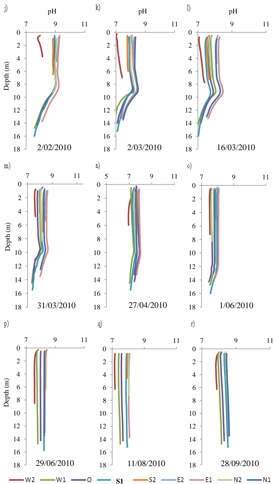
Figures 3.8j-r: pH for all stations from 02 February 2010 to 28 September 2010.
