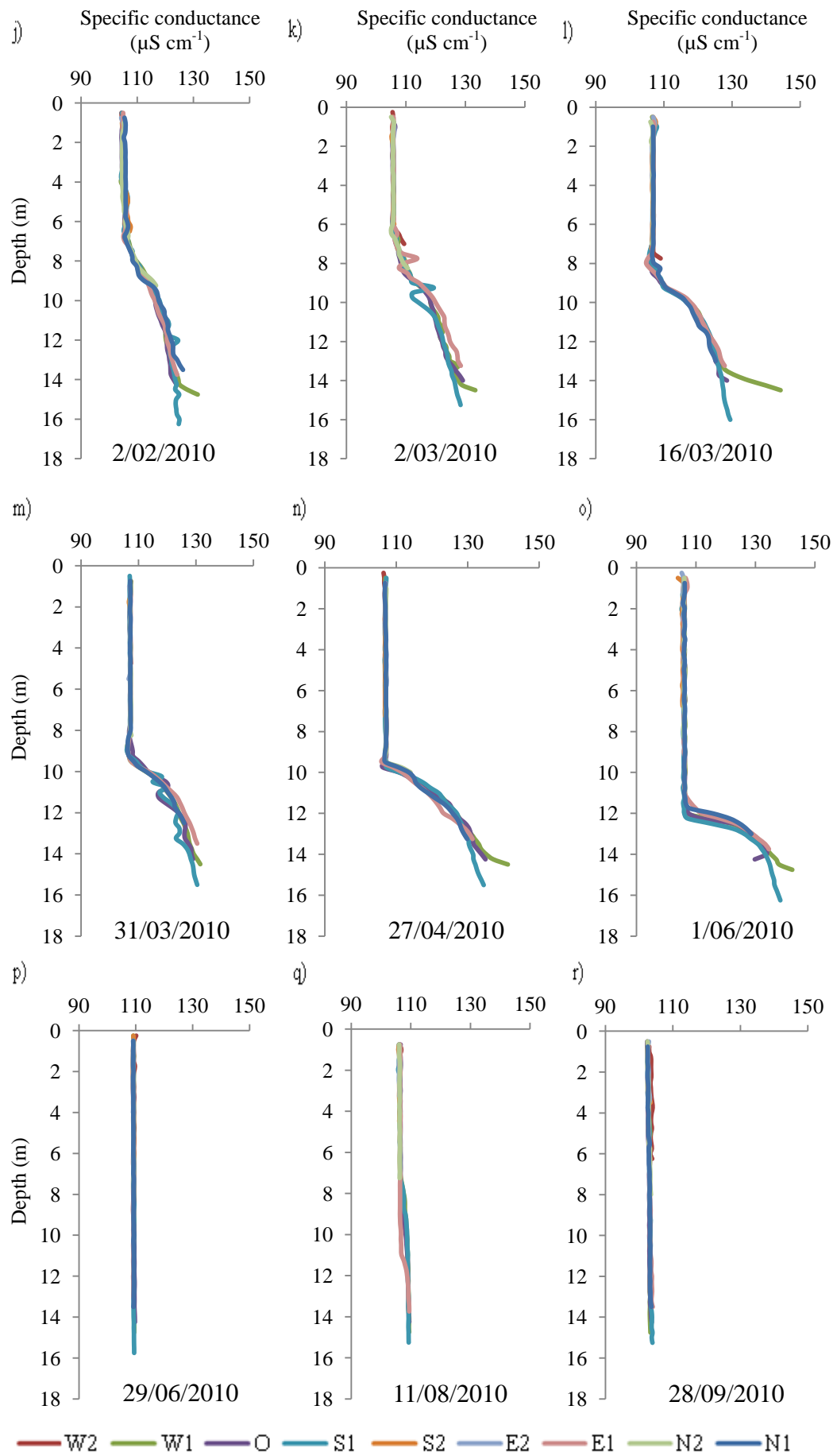
Figures 3.9j-r: Specific conductance for all stations from 02 February 2010 to 28 September 2010.
