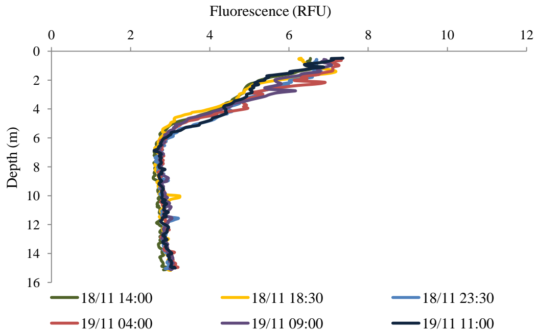
Figure 4.6: Fluorescence on 18-19 November 2010. Date and time (h) of each profile are given in inset.
