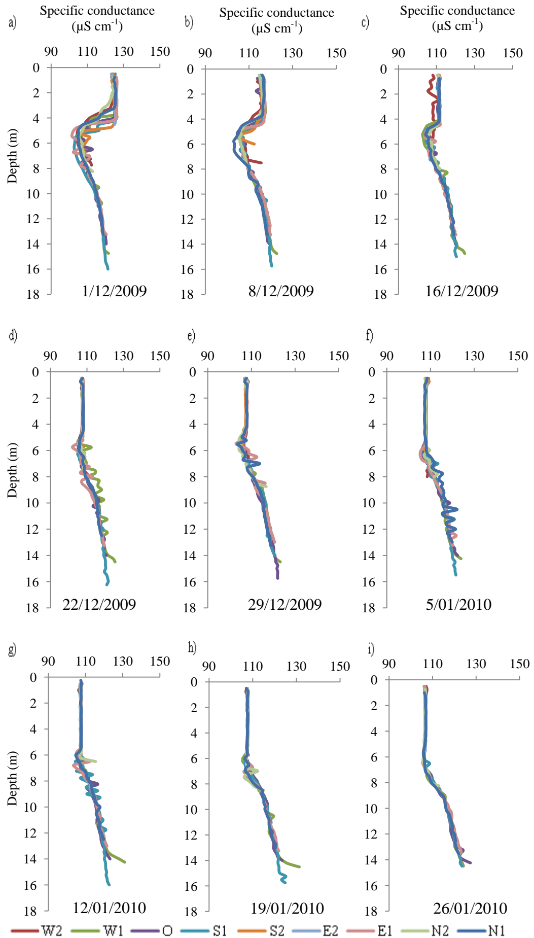
Figures 3.9a-i: Specific conductance for all stations from 01 December 2009 to 26 January 2010
