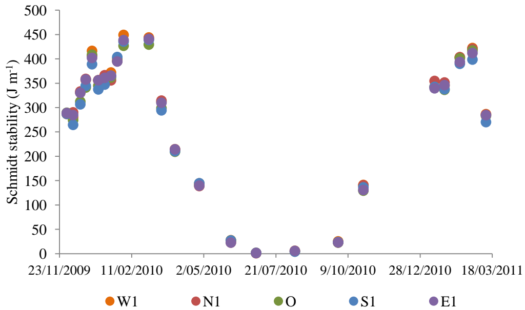
Figure 3.2: Schmidt stability at deep stations (station names are given on the inset) from 01 December 2009 – 11 March 2011.
