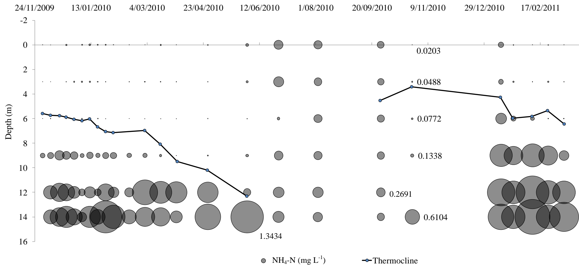
Figure 3.10a: Concentrations of \text{NH}_4\text{-N} at 0, 3, 6, 9, 12 and 14 m depth in samples taken from 01 December 2009 - 11 March 2011, and thermocline depth. Reference values are provided next to several sample points (mg \text{L}^{-1} ).
