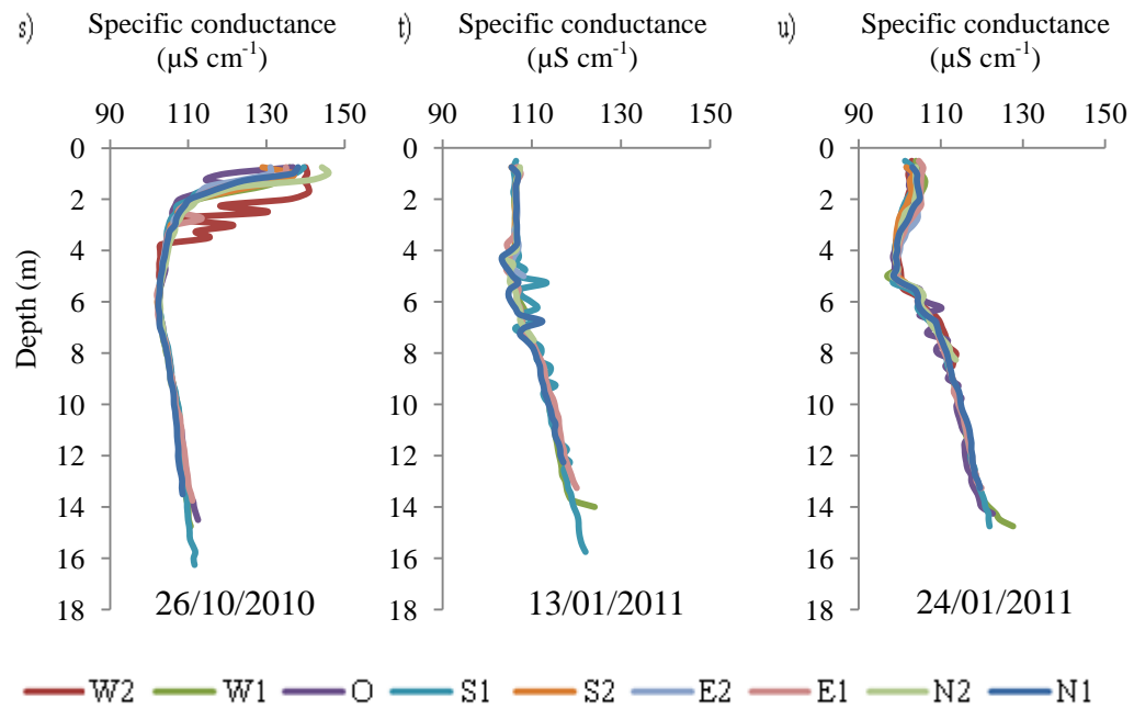
Figures 3.9s-u: Specific conductance for all stations from 26 October 2010 to 24 January 2011.
