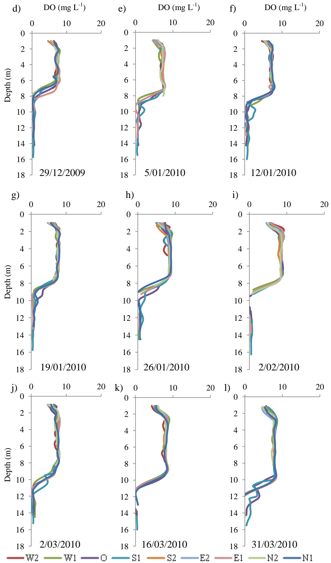
Figures 3.7d-l: Dissolved oxygen profiles for all stations from 29 December 2009 to 31 March 2010.
