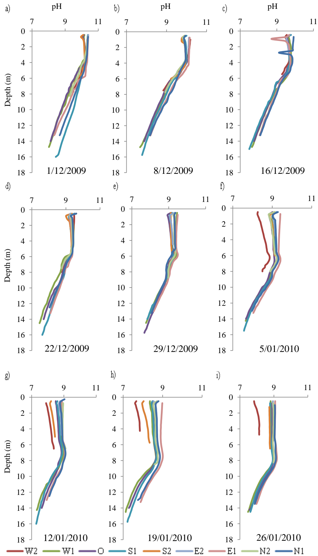
Figures 3.8a-i: pH for all stations from 01 December 2009 to 26 January 2010.
