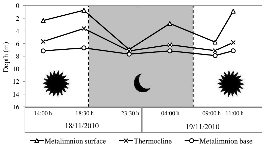
Figure 4.2: Depth of the upper and lower metalimnion and of the thermocline on 18-19 November 2010. Date and time (h) of each profile are given in inset.
