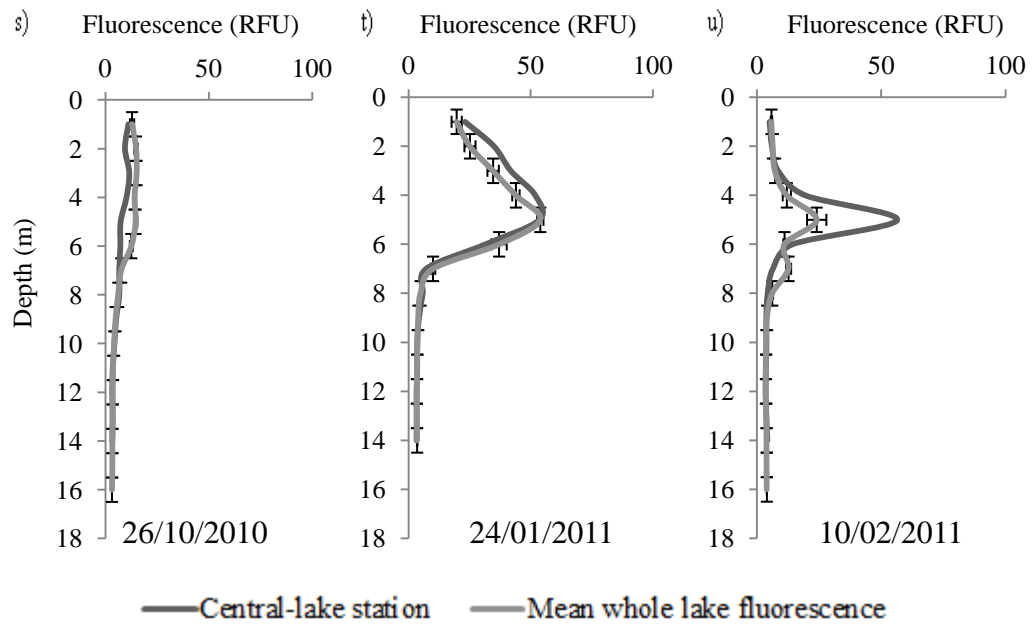
Figures 3.11s-u: Fluorescence (RFU) at central station and whole lake mean fluorescence with standard error from 26 October 2010 to 10 February 2011.
