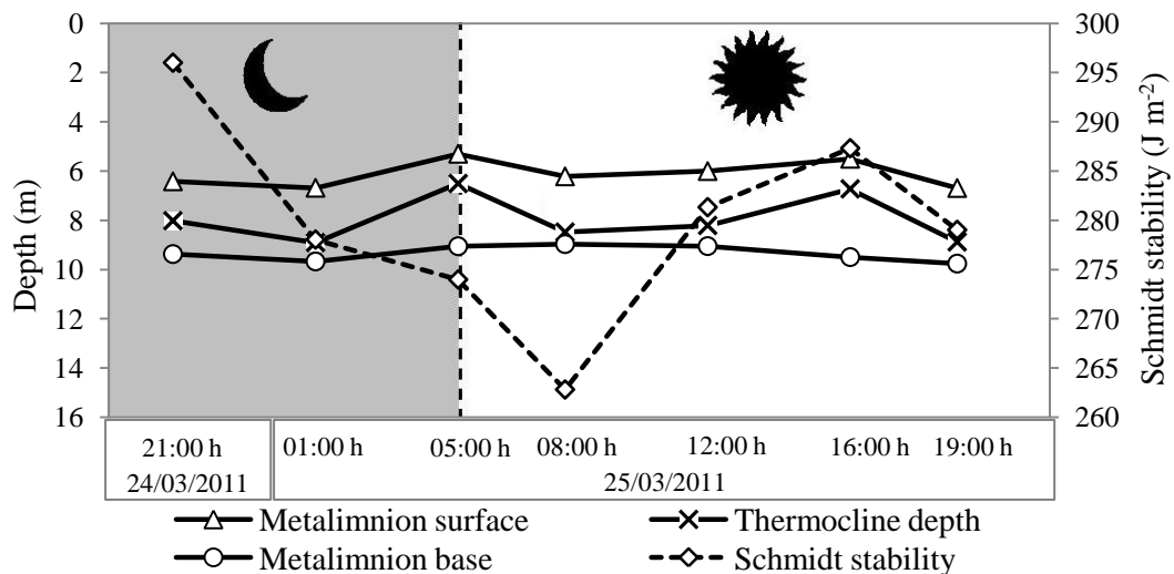
Figure 4.8: Depth of the upper and lower metalimnion, the thermocline and Schmidt stability on 24-25 March 2011. Date and time (h) of each profile are given in inset.
