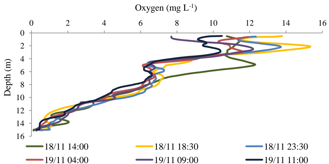
Figure 4.3: Dissolved oxygen concentrations on 18-19 November 2010. Date and time (h) of each profile are given in inset.
