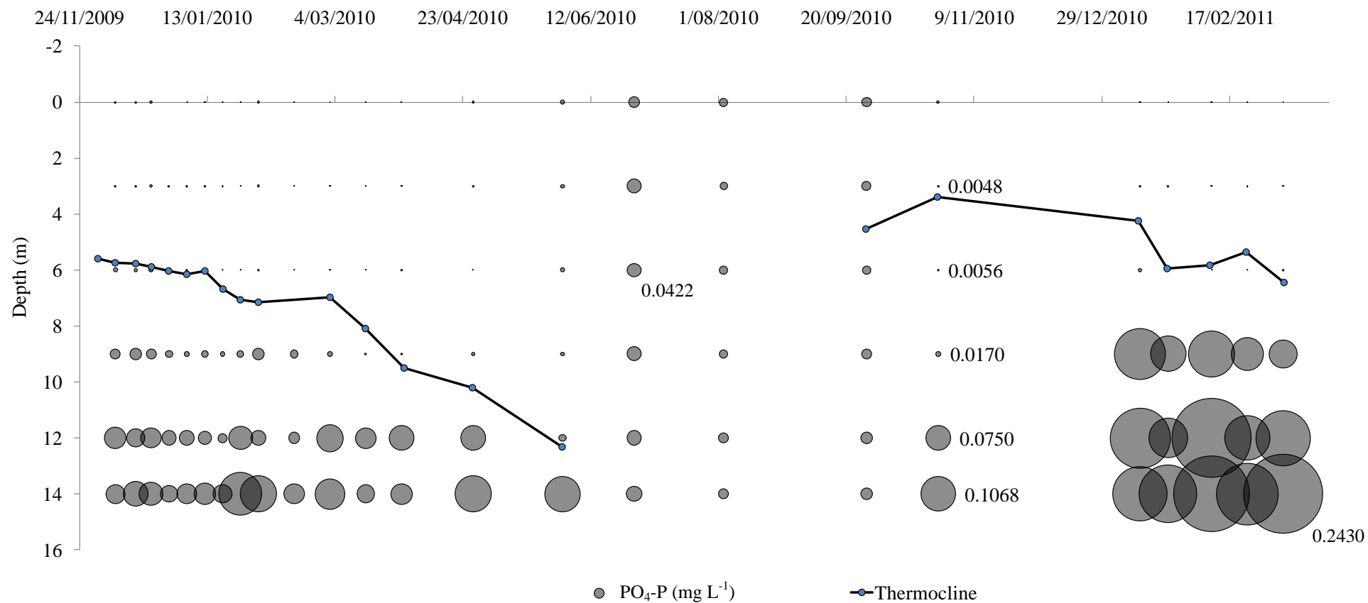
Figure 3.10c: Concentrations of \text{PO}_4\text{-P} at 0, 3, 6, 9, 12 and 14 m depth in samples taken from 08 December 2009 - 11 March 2011, and thermocline depth. Reference values are given next to several sample points ( \text{mg L}^{-1} ).
