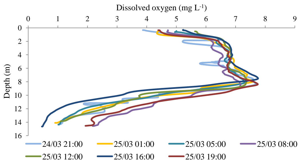
Figure 4.9: Dissolved oxygen concentrations on 24-25 March 2011. Date and time (h) of each profile are given in inset.
