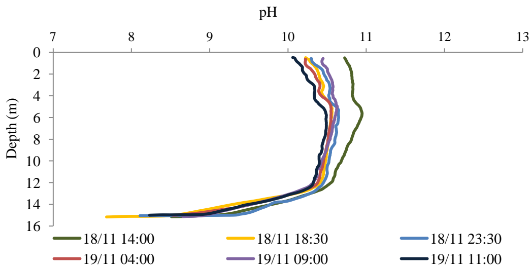
Figure 4.5: pH profiles on 18-19 November 2010. Date and time (h) of each profile are given in inset.
