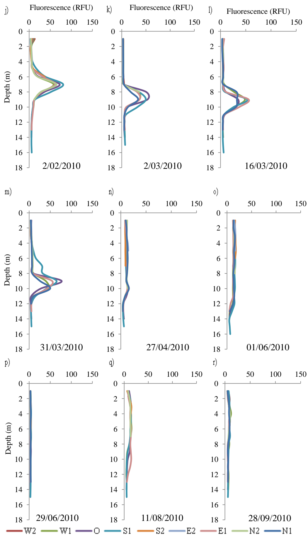
Figures 3.6j-r: Fluorescence profiles for all stations from 02 February 2010 – 28 September 2010.
