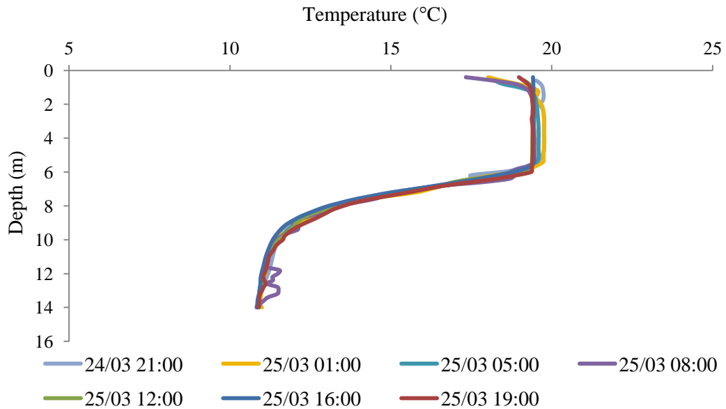
Figure 4.7: Temperature profiles on 24-25 March 2011. Date and time (h) of each profile are given in inset.
