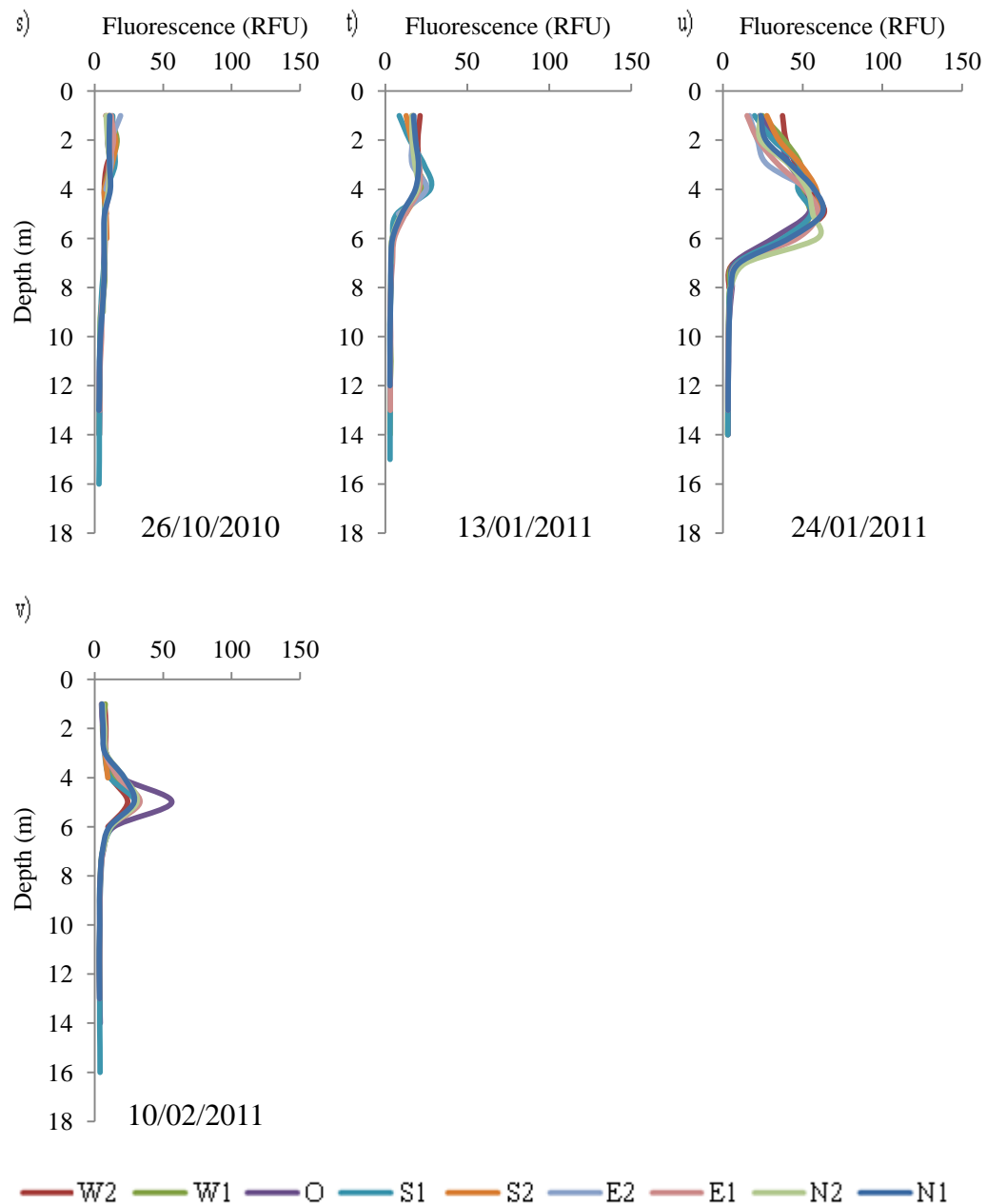
Figures 3.6s-v: Fluorescence profiles for all stations from 26 October 2010 – 10 February 2011.
