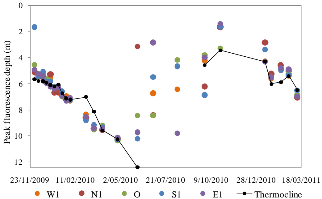
Figure 3.3: Depth of peak fluorescence with mean thermocline depth at deep stations (station names are given on the inset) from 01 December 2009 – 11 March 2011. No thermocline was present from 01 June 2010 until 28 September 2010.
