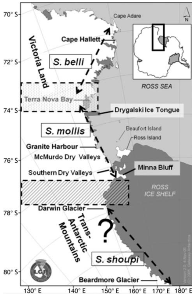
Fig. 1. Location of the Victoria Land Transantarctic latitudinal gradient (inset) showing the known, approximate distributions for three species of Stereotydeus ( S. belli , S. mollis , S. shoupi ). Place names are referred to in the text. McMurdo Dry Valleys include Victoria, Wright and Taylor valleys; Southern Dry Valleys include Garwood, Marshall and Miers valleys. The stippled area indicates an area of overlap in the distributions of S. belli and S. mollis . The hatched area indicates an ice-covered area that occurs between the ranges of S. mollis and S. shoupi . The question mark (“?”) indicates an area where limited information is currently available on the distribution of S. shoupi .
