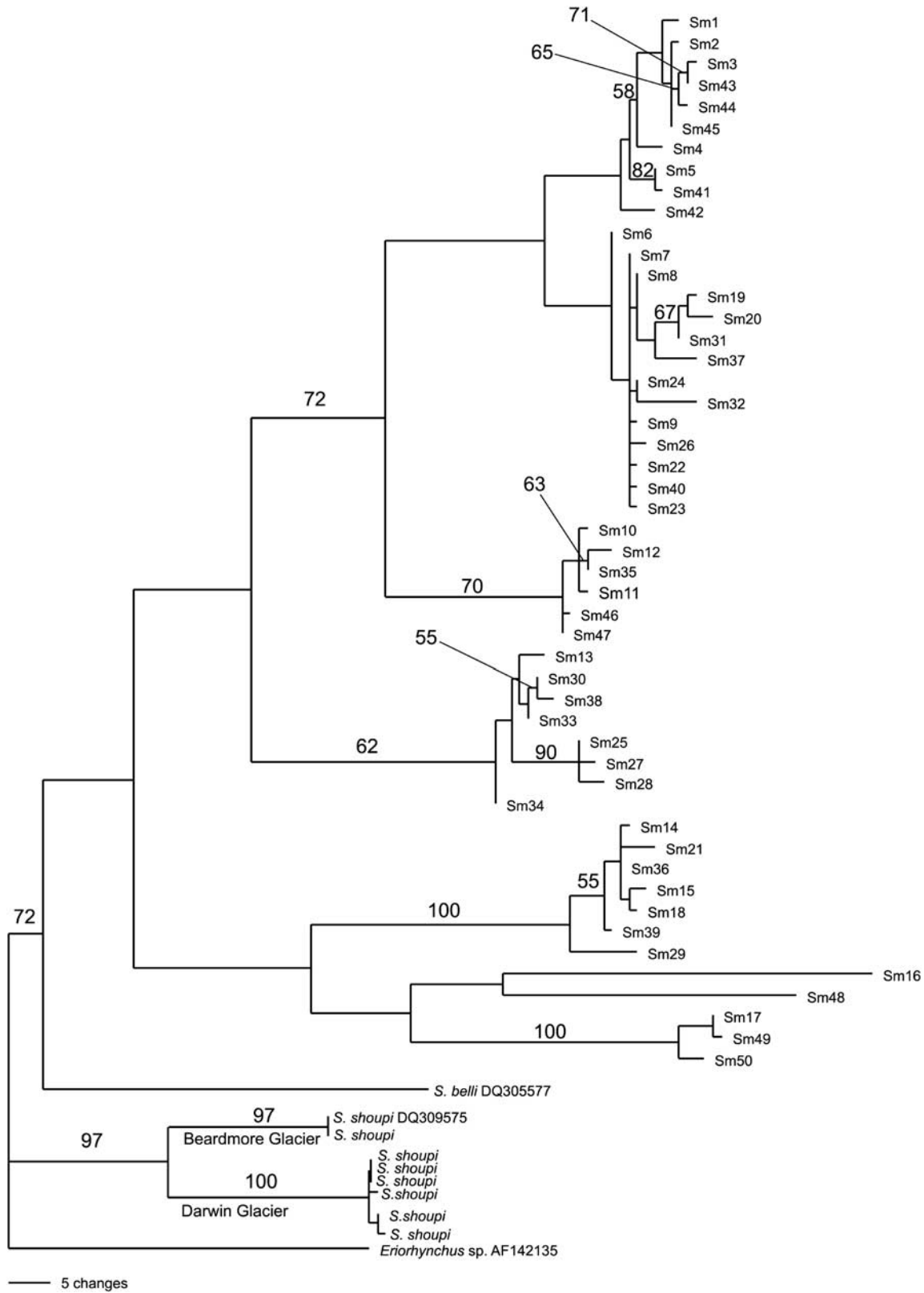
Fig. 3. Maximum likelihood phylogram based upon the substitution model HKY+I+ \Gamma (-lnL = 3158.0623 (AIC); Ti/tv ratio = 2.8729 I = 0.5320 \Gamma = 0.7250; with base frequencies set to A = 0.4094 C = 0.0919 G = 0.1180 T = 0.3807) derived from jModeltest (see methods), using a 504 bp fragment of the mtDNA (COI) gene from all available Stereotydeus sequences from Victoria Land and the central Transantarctic Mountains. Haplotype codes refer to those provided in Table I.
