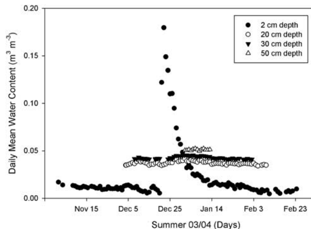
Fig. 2. Daily mean soil liquid water contents in the active layer for the Wright Valley soil climate station in summer 2003–04.
