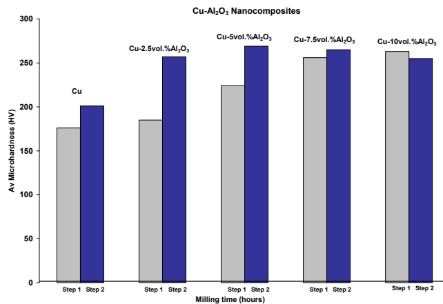
Fig. 1: The average microhardness of Cu powder particles and Cu-(2.5-10)vol.%Al 2 O 3 nanocomposite powder particles produced by HEMM after Step 1 and Step 2 respectively.
