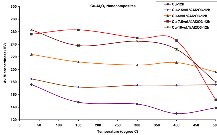
Fig. 2: Average microhardness of Cu powder particles and Cu-(2.5-10)vol.%Al 2 O 3 nanocomposite powder particles produced with 12 hours of milling (Step 1) as a function of annealing temperature.
