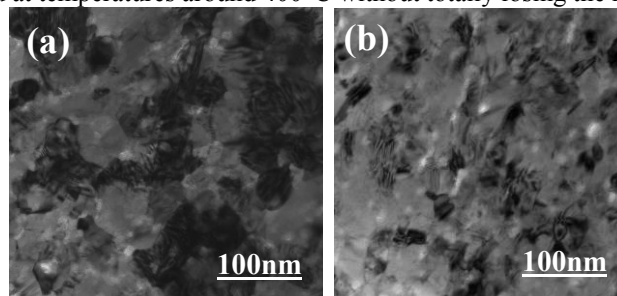
Fig. 5: TEM Bright field images of Cu-10vol.%Al 2 O 3 produced with Step 1 of HEMM after annealing at 150°C.
