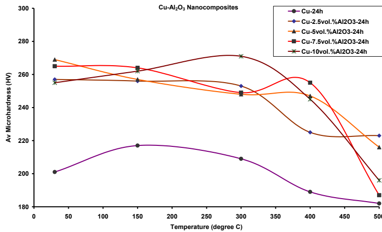
Fig. 3: The average microhardness of Cu powder particles and Cu-(2.5-10)vol.%Al 2 O 3 nanocomposite powder particles produced with 24 hours of milling (Step 2) as a function of annealing temperature.
