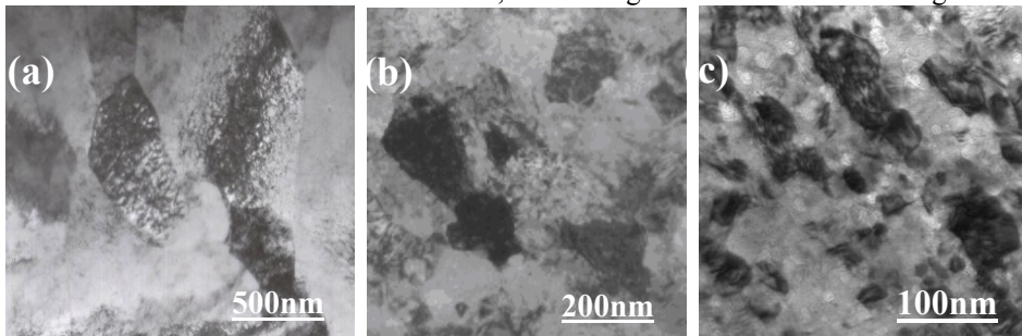
Fig. 4: TEM Bright field images produced with Step 1 of HEMM (a) Cu-2.5vol.%Al 2 O 3 (b) Cu-5vol.%Al 2 O 3 (c) Cu-7.5vol.%Al 2 O 3 .
