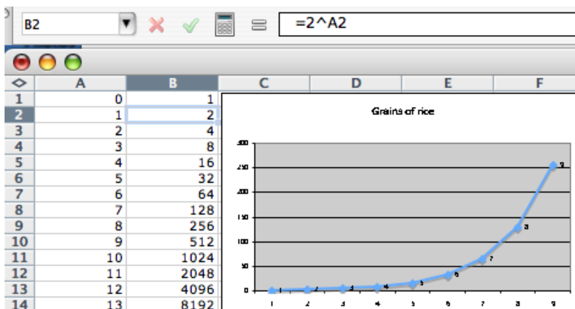
Figure 1: Multi-representations of data from Rice Mate investigation involving powers of two.
