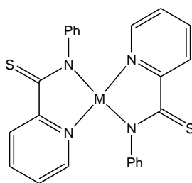
7a M=Pd 7b M=Pt
