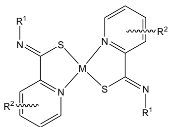
6a M=Pd, R 1 = o -tolyl, R 2 =H 6b M=Pd, R 1 =Me, R 2 =4-Me 6c M=Pt, R 1 = o -tolyl, R 2 =H
