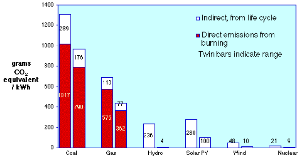
Chart 1 Greenhouse gas emission from electricity production
