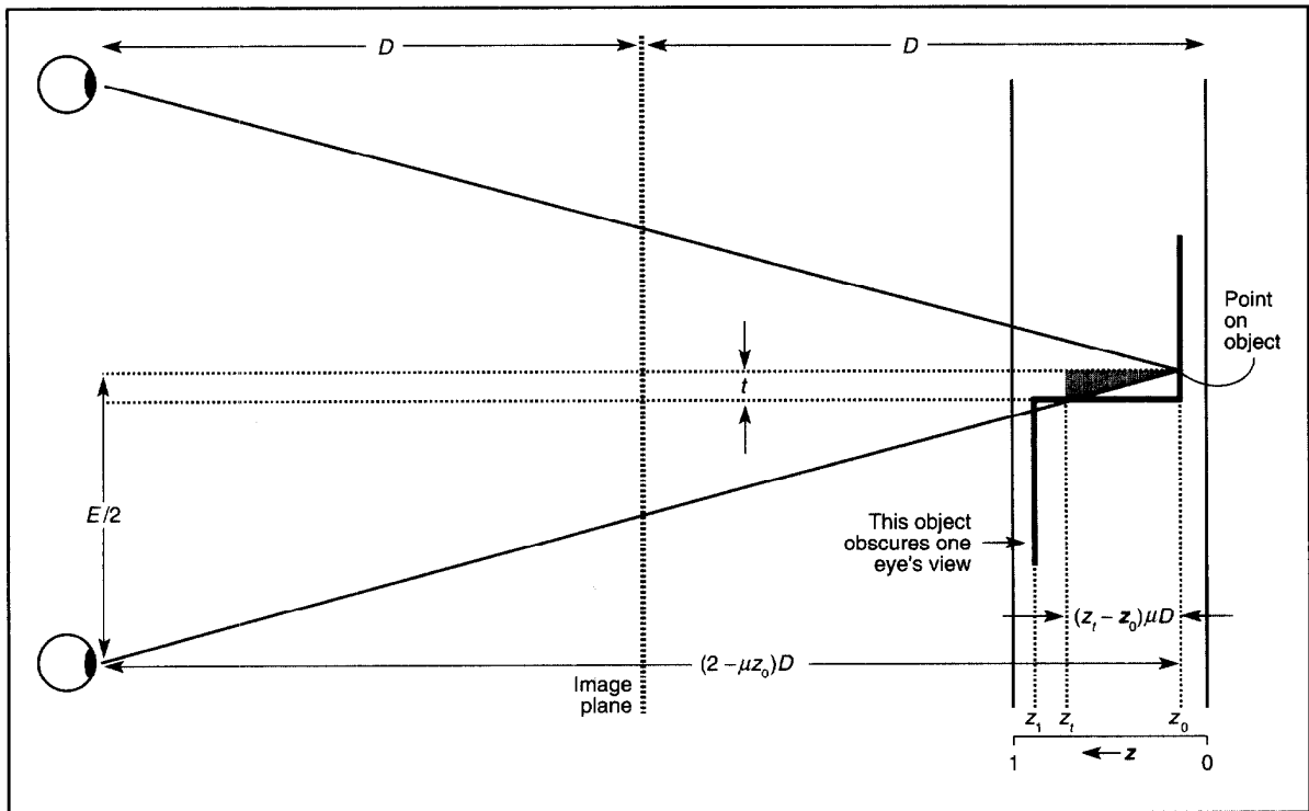
Figure 4. The geometry for hidden-surface removal, which is performed by the algorithm.
