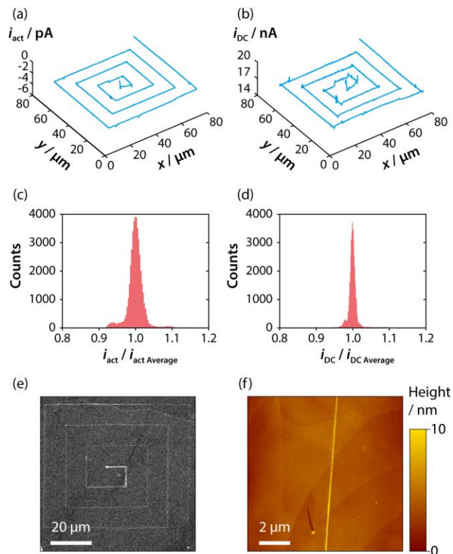
Figure 6. SECCM maps of: (a) surface activity ( i_{act} ) and (b) DC component of conductance current ( i_{DC} ) for the diffusion-limited reduction of 100 \mu\text{M} AQDS in 0.1 M \text{HClO}_4 during reactive line-patterning on AM HOPG, at a scan speed of 1 \mu\text{m s}^{-1} . Corresponding histograms of the spread of currents are shown in (c) and (d), respectively. (e) FE-SEM image showing the deposited AQDS line pattern. (f) AFM image of part of the pattern.
