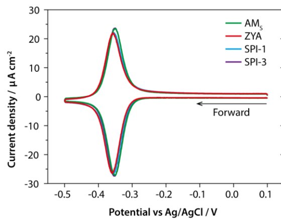
Figure 1. CVs ( 0.1 \text{ V s}^{-1} ) for the reduction of 10 \text{ } \mu\text{M} AQDS in 0.1 \text{ M HClO}_4 on four grades of freshly cleaved HOPG: AM 5 (Scotch tape cleaved), ZYA, SPI-1 and SPI-3.
