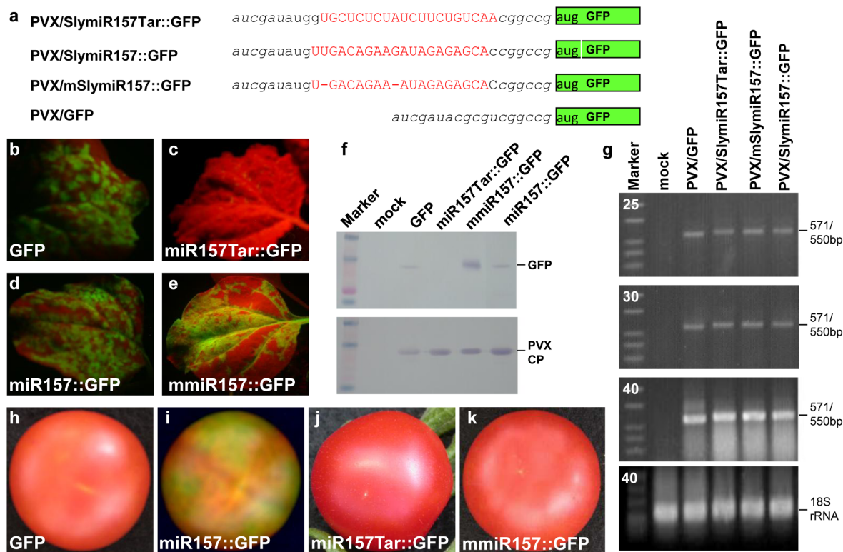
Figure 4 | miRNA target – GFP reporter expression assay. (a) PVX-based miRNA target – GFP reporter expression vectors. (b–e) Nicotiana benthamiana leaves were inoculated with PVX/GFP (GFP, b), PVX/SlymiR157Tar::GFP (miR157Tar::GFP, c), PVX/SlymiR157::GFP (miR157::GFP, d) or PVX/mSlymiR157::GFP (mmiR157::GFP, e). Photographs were taken under long-wavelength UV light at 7 days post inoculation. GFP fluorescence is green and leaf auto-fluorescence shows red. (f) Western blot detection of GFP and PVX coat protein (CP) in mock- or PVX-inoculated leaf tissues using antibody raised specifically against GFP and the viral CP. Positions of GFP and PVX CP are indicated. (g) Detection of recombinant PVX::miRNA target::GFP RNA in same leaf samples as used in Western blot by semi-qRT-PCR. The positions and sizes of amplified fragments and the number of PCR cycles are indicated. 18S rRNA was used as controls. (h–k) AC fruits were injected with PVX/GFP (h), PVX/SlymiR157::GFP (i), PVX/SlymiR157Tar::GFP (j) or PVX/mSlymiR157::GFP (k). Non-ripening sectors show green. Fruits were photographed at 7 days after breaker.
