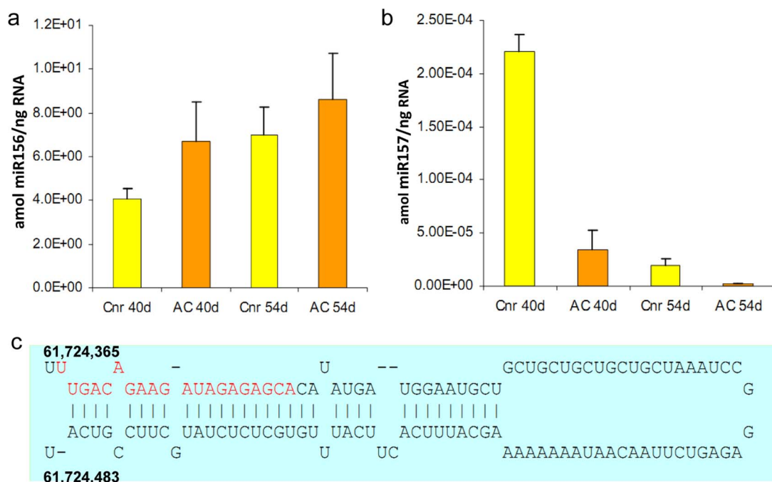
Figure 1 | Differential and developmental regulation of SlymiR157 in tomato fruits. (a) Transcript profiles of SlymiR156 in wild type Ailsa Craig (AC) and Cnr epimutant fruits at breaker (40 days post anthesis, dpa) and at 54 dpa (d). (b) Differential and developmental expression of SlymiR157 in AC and Cnr fruits. The amount of SlymiR157 was significantly higher at 40 dpa than 54 dpa in Cnr fruits. A similar trend of the SlymiR157 level was also found in AC and Cnr fruits, but expression of SlymiR157 decreased markedly in AC than Cnr fruits at the same stage of the ripening process. (c) Stem-loop structure of the pre-SlymiR157 RNA molecule. The genome coordinates on tomato Chromosome 3 are indicated.
